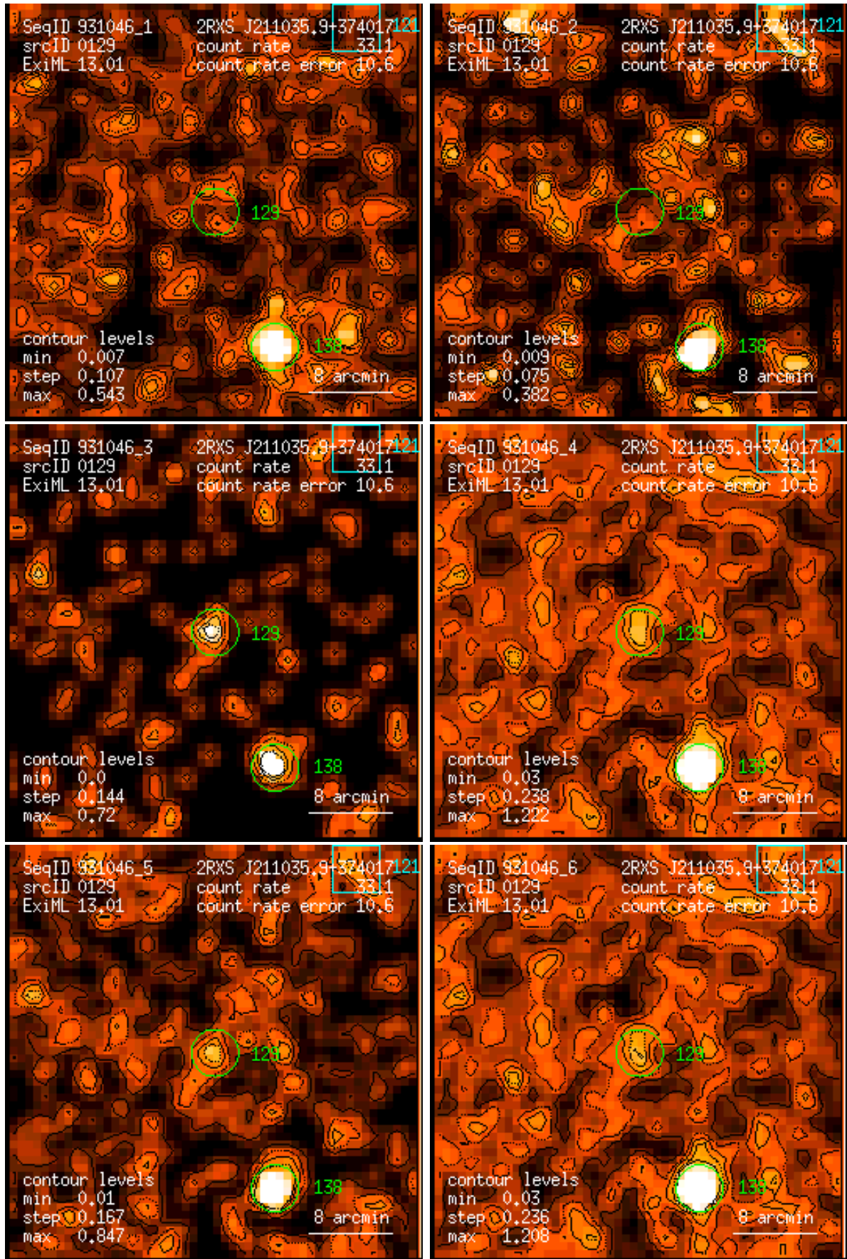
Figure 129: RASS 931046: detection 0129: band rate images, Gaussian filter: (1) PSPC channels 11 – 41, (2) 52 – 90, (3) 91 – 201, (4) 11 – 235, (5) 52 – 201, (6) 11 – 201. Broad band rates in counts/ks. Band rate contour levels in counts/ks/arcmin 2 .
