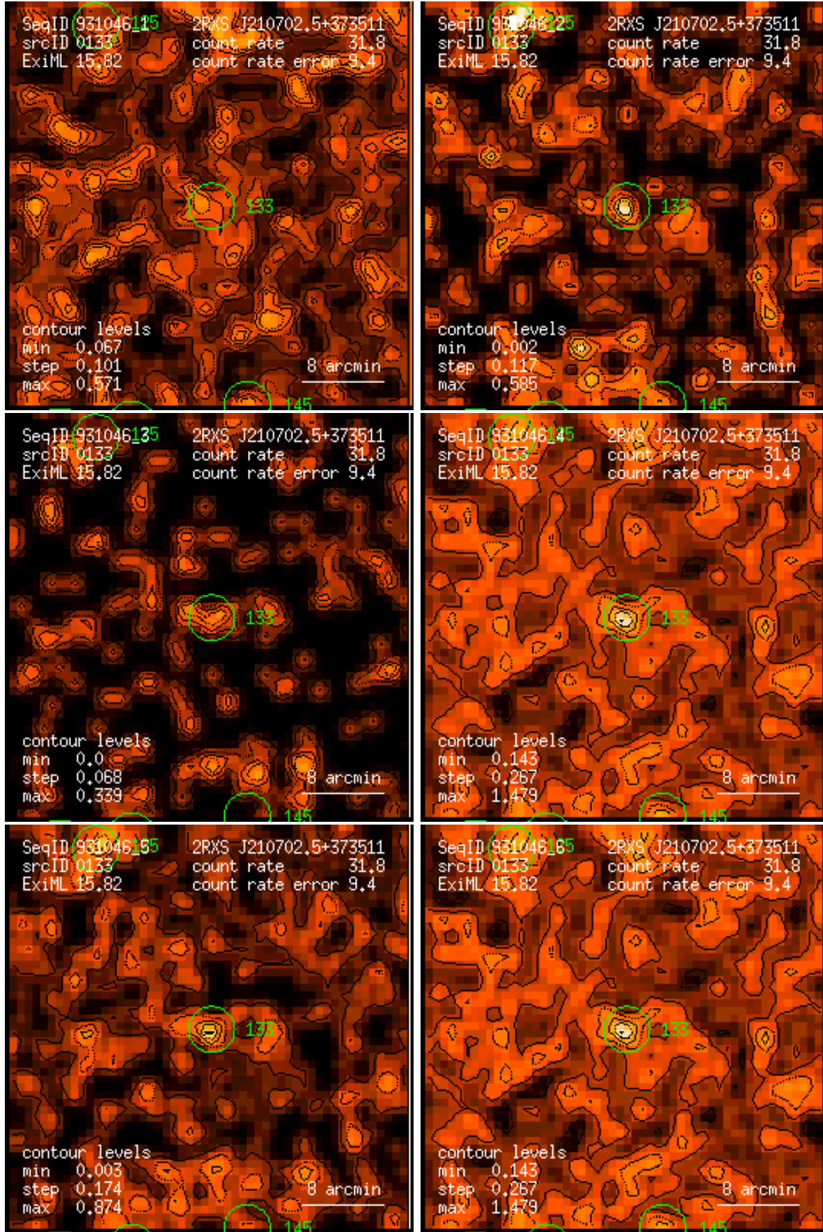
Figure 133: RASS 931046: detection 0133: band rate images, Gaussian filter: (1) PSPC channels 11 – 41, (2) 52 – 90, (3) 91 – 201, (4) 11 – 235, (5) 52 – 201, (6) 11 – 201. Broad band rates in counts/ks. Band rate contour levels in counts/ks/arcmin 2 .
