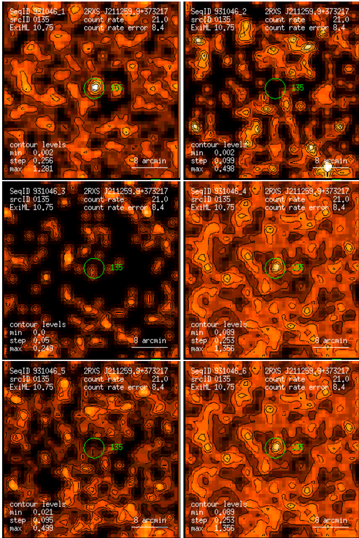
Figure 135: RASS 931046: detection 0135: band rate images, Gaussian filter: (1) PSPC channels 11 – 41, (2) 52 – 90, (3) 91 – 201, (4) 11 – 235, (5) 52 – 201, (6) 11 – 201. Broad band rates in counts/ks. Band rate contour levels in counts/ks/arcmin 2 .
