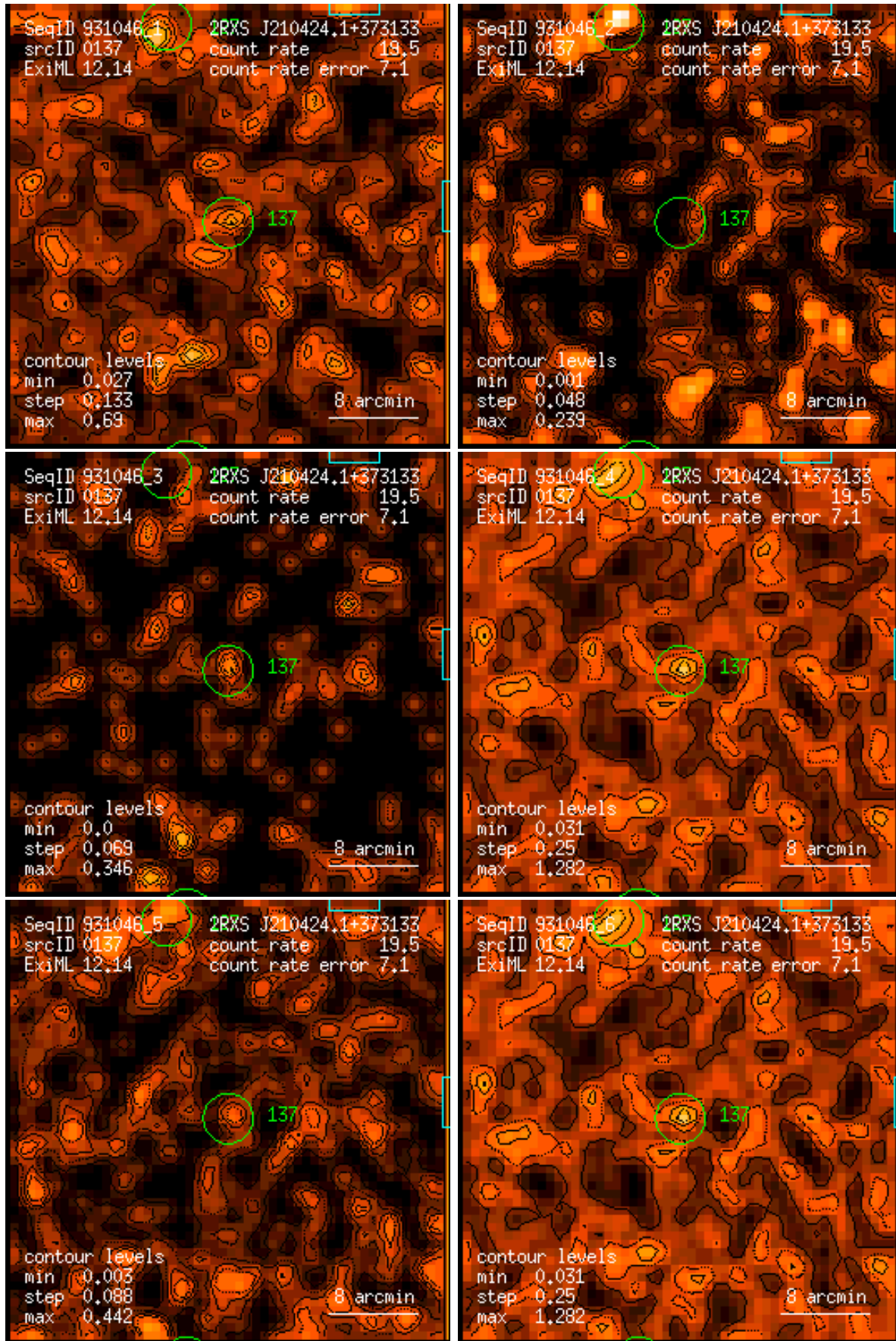
Figure 137: RASS 931046: detection 0137: band rate images, Gaussian filter: (1) PSPC channels 11 – 41, (2) 52 – 90, (3) 91 – 201, (4) 11 – 235, (5) 52 – 201, (6) 11 – 201. Broad band rates in counts/ks. Band rate contour levels in counts/ks/arcmin 2 .
