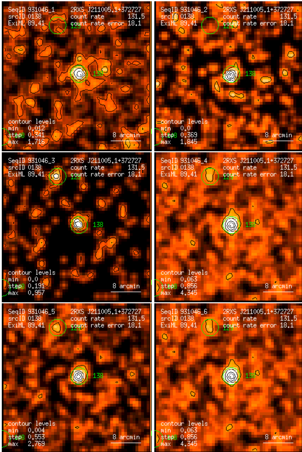
Figure 138: RASS 931046: detection 0138: band rate images, Gaussian filter: (1) PSPC channels 11 – 41, (2) 52 – 90, (3) 91 – 201, (4) 11 – 235, (5) 52 – 201, (6) 11 – 201. Broad band rates in counts/ks. Band rate contour levels in counts/ks/arcmin 2 .
