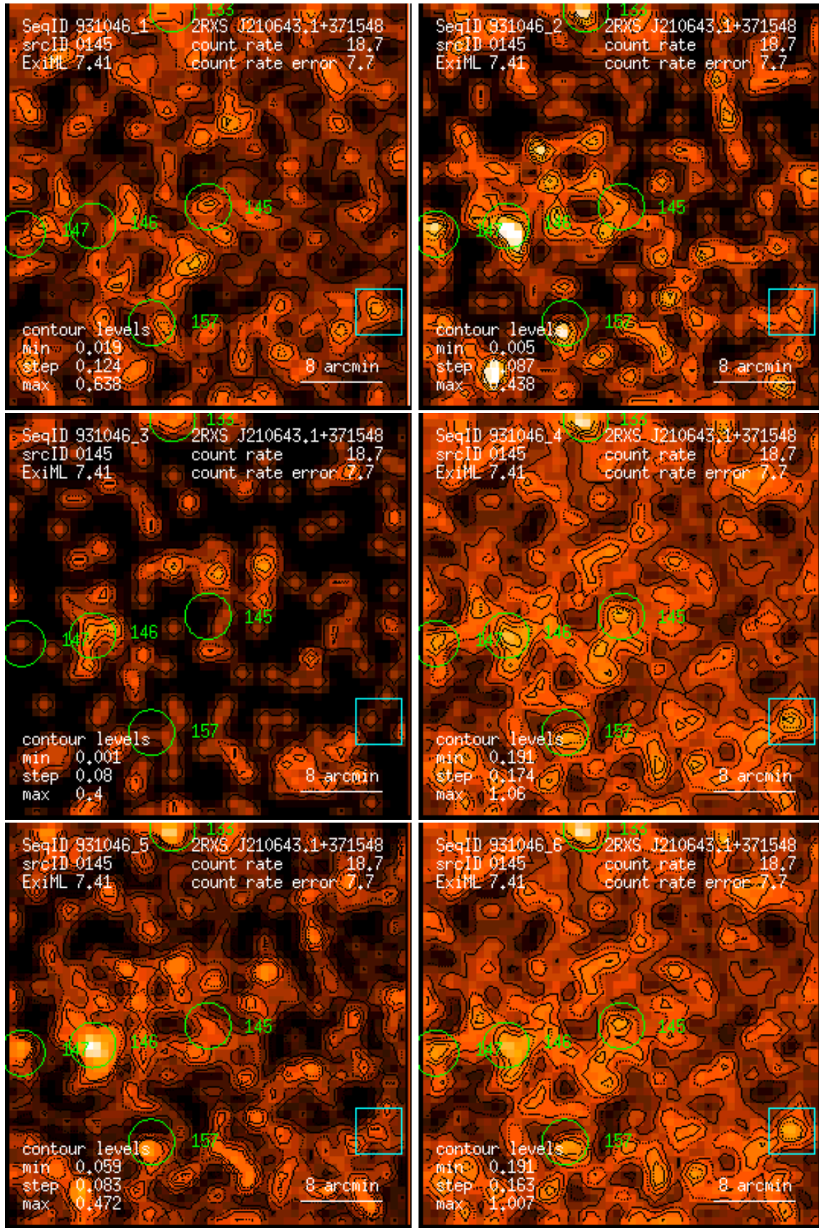
Figure 145: RASS 931046: detection 0145: band rate images, Gaussian filter: (1) PSPC channels 11 – 41, (2) 52 – 90, (3) 91 – 201, (4) 11 – 235, (5) 52 – 201, (6) 11 – 201. Broad band rates in counts/ks. Band rate contour levels in counts/ks/arcmin 2 .
