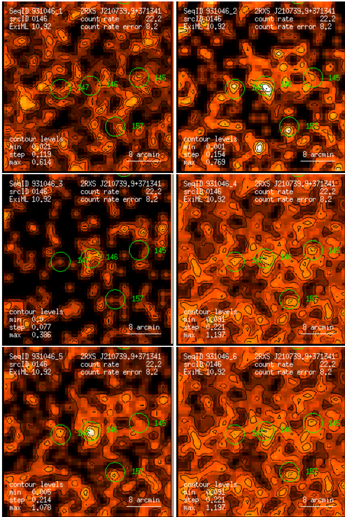
Figure 146: RASS 931046: detection 0146: band rate images, Gaussian filter: (1) PSPC channels 11 – 41, (2) 52 – 90, (3) 91 – 201, (4) 11 – 235, (5) 52 – 201, (6) 11 – 201. Broad band rates in counts/ks. Band rate contour levels in counts/ks/arcmin 2 .
