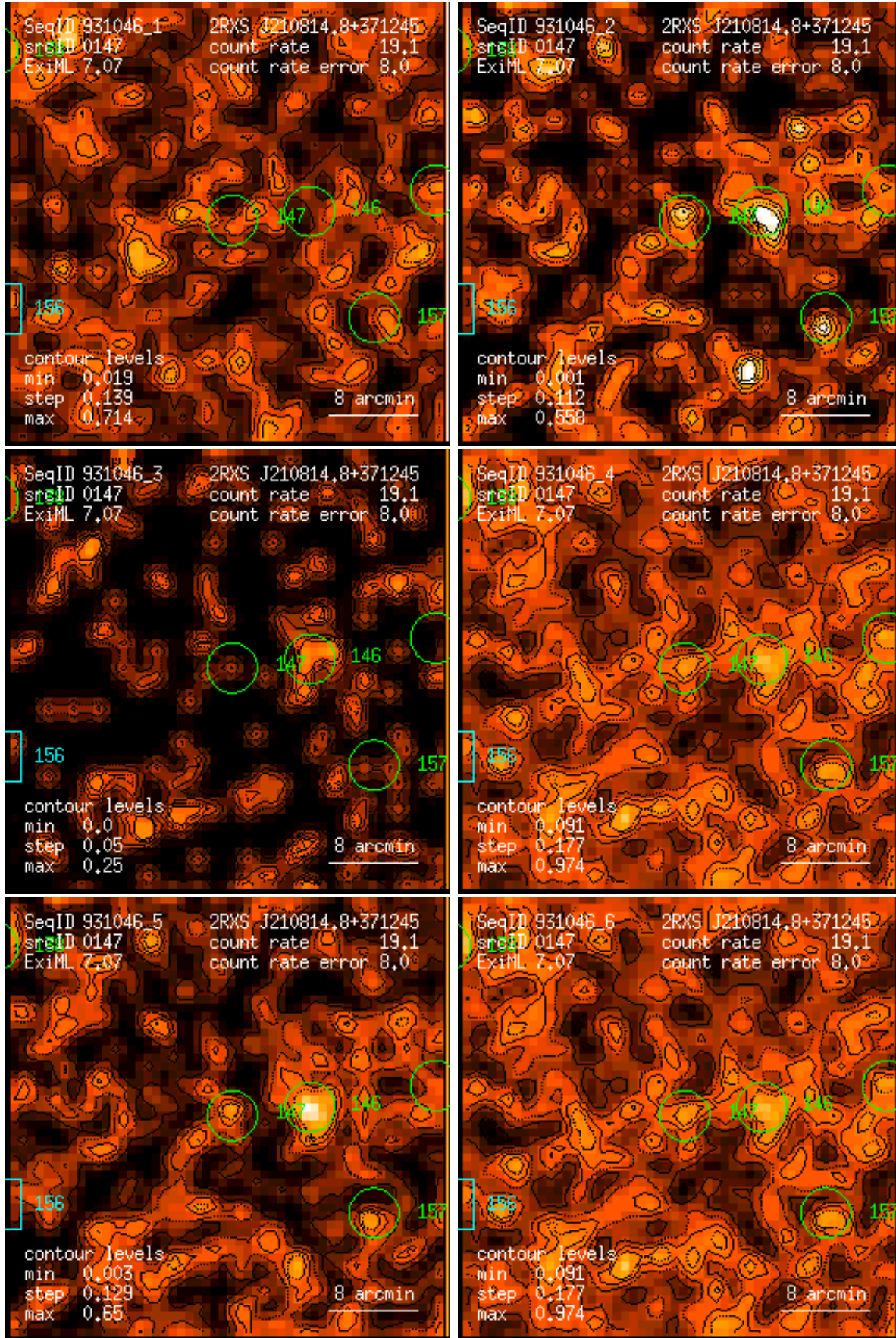
Figure 147: RASS 931046: detection 0147: band rate images, Gaussian filter: (1) PSPC channels 11 – 41, (2) 52 – 90, (3) 91 – 201, (4) 11 – 235, (5) 52 – 201, (6) 11 – 201. Broad band rates in counts/ks. Band rate contour levels in counts/ks/arcmin 2 .
