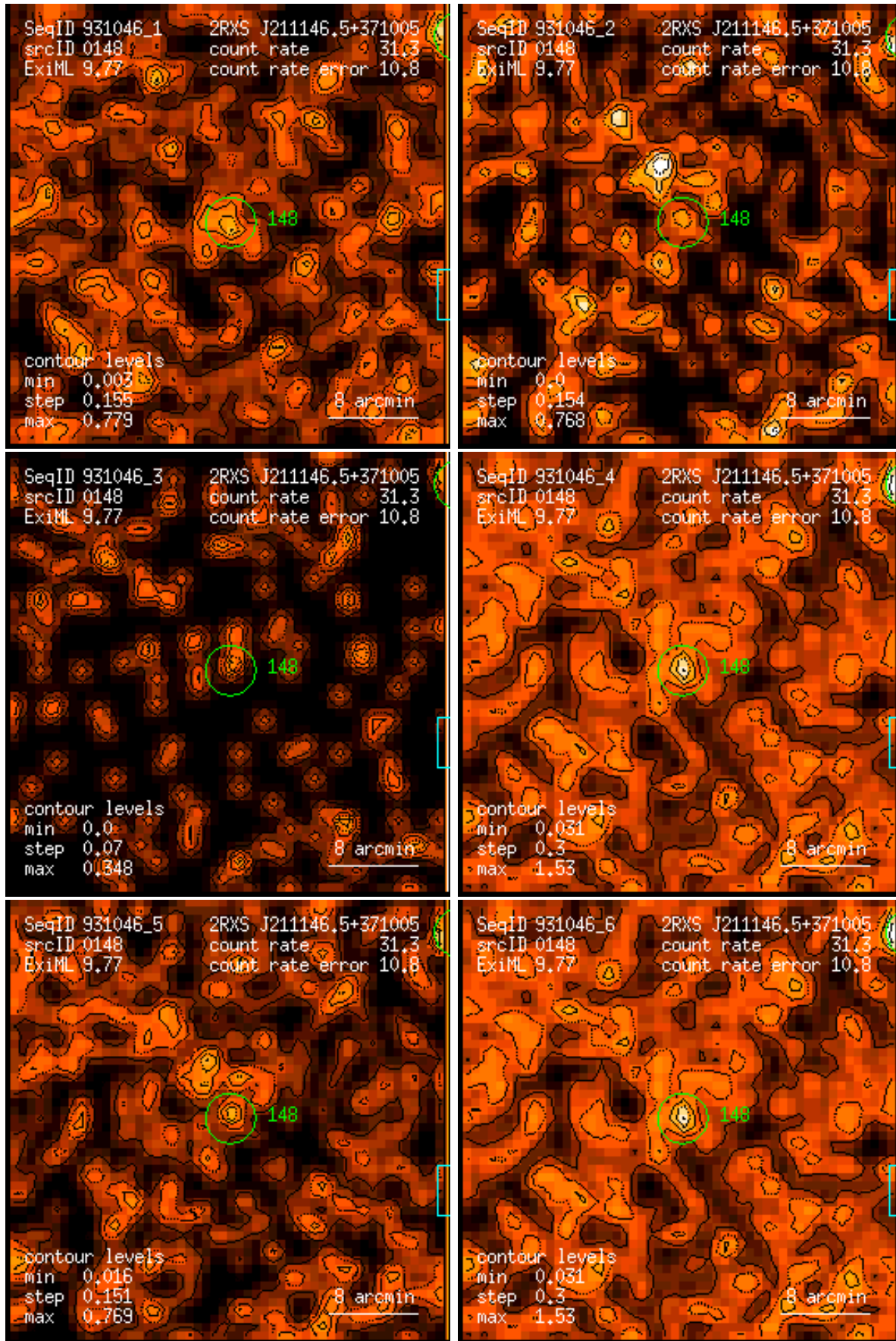
Figure 148: RASS 931046: detection 0148: band rate images, Gaussian filter: (1) PSPC channels 11 – 41, (2) 52 – 90, (3) 91 – 201, (4) 11 – 235, (5) 52 – 201, (6) 11 – 201. Broad band rates in counts/ks. Band rate contour levels in counts/ks/arcmin 2 .
