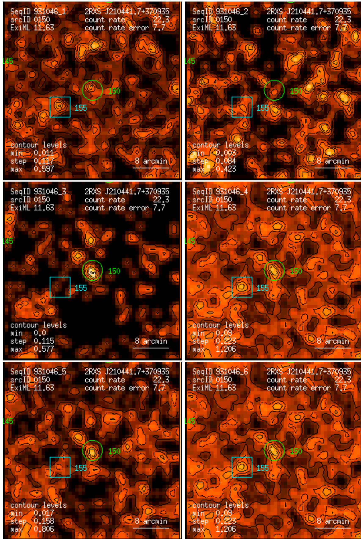
Figure 150: RASS 931046: detection 0150: band rate images, Gaussian filter: (1) PSPC channels 11 – 41, (2) 52 – 90, (3) 91 – 201, (4) 11 – 235, (5) 52 – 201, (6) 11 – 201. Broad band rates in counts/ks. Band rate contour levels in counts/ks/arcmin 2 .
