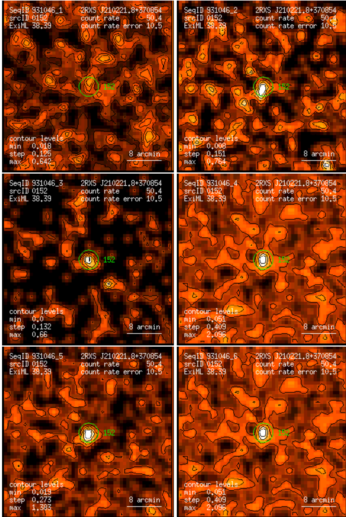
Figure 152: RASS 931046: detection 0152: band rate images, Gaussian filter: (1) PSPC channels 11 – 41, (2) 52 – 90, (3) 91 – 201, (4) 11 – 235, (5) 52 – 201, (6) 11 – 201. Broad band rates in counts/ks. Band rate contour levels in counts/ks/arcmin 2 .
