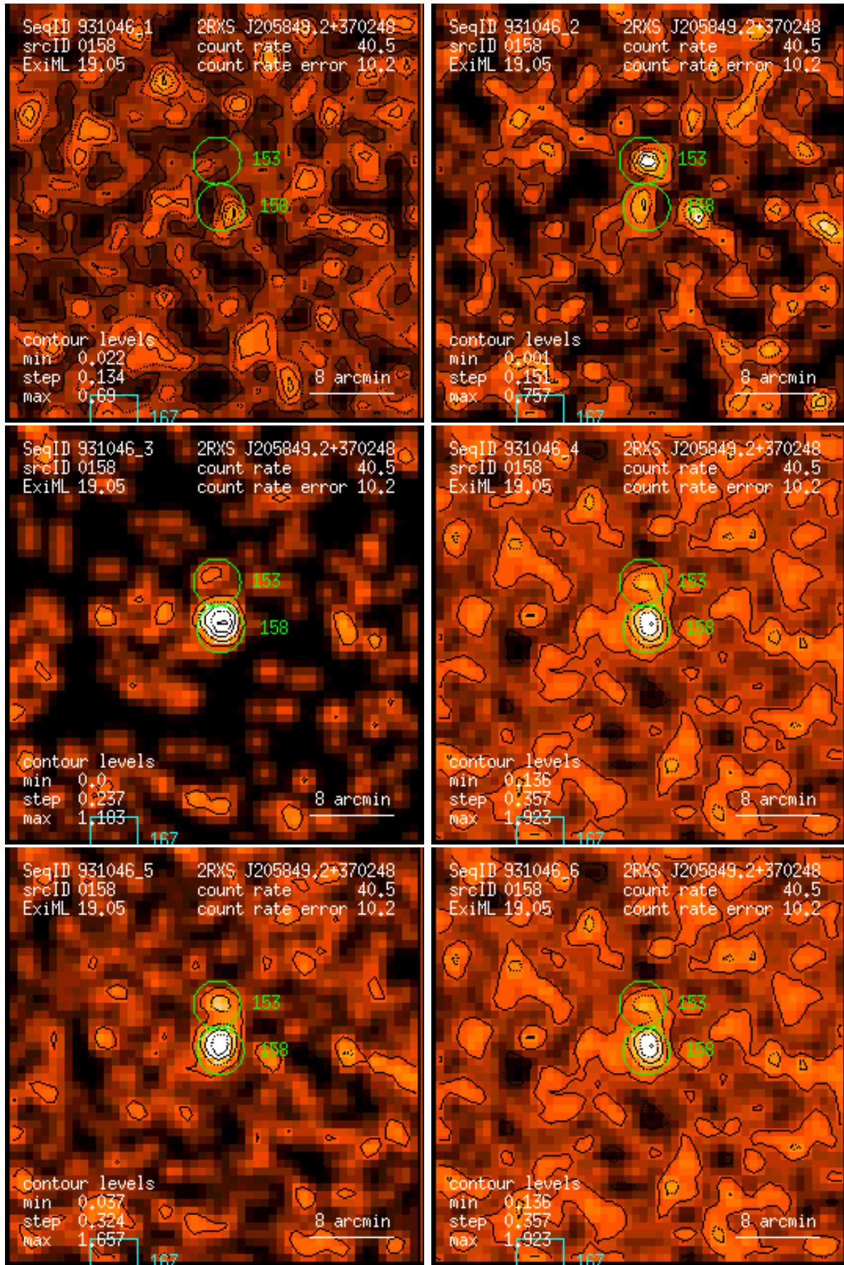
Figure 158: RASS 931046: detection 0158: band rate images, Gaussian filter: (1) PSPC channels 11 – 41, (2) 52 – 90, (3) 91 – 201, (4) 11 – 235, (5) 52 – 201, (6) 11 – 201. Broad band rates in counts/ks. Band rate contour levels in counts/ks/arcmin 2 .
