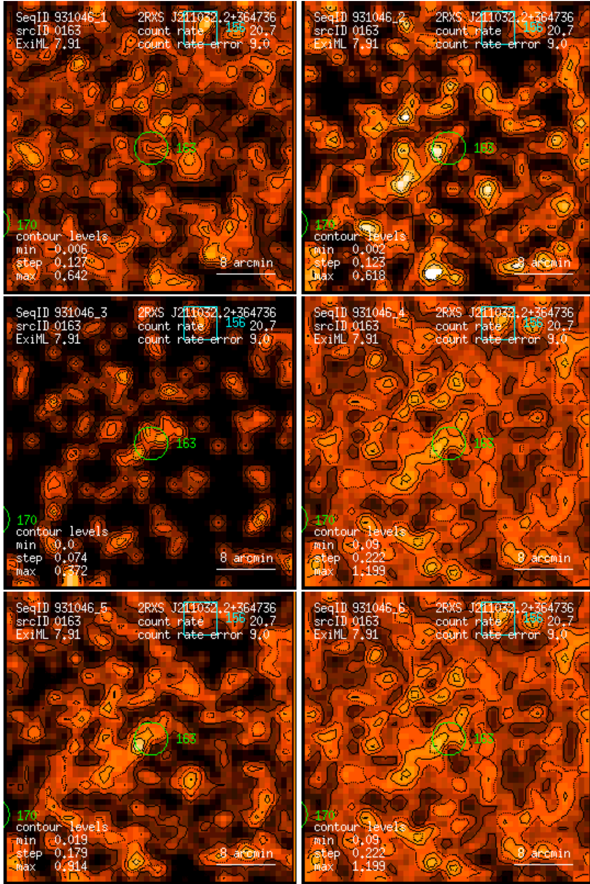
Figure 163: RASS 931046: detection 0163: band rate images, Gaussian filter: (1) PSPC channels 11 – 41, (2) 52 – 90, (3) 91 – 201, (4) 11 – 235, (5) 52 – 201, (6) 11 – 201. Broad band rates in counts/ks. Band rate contour levels in counts/ks/arcmin 2 .
