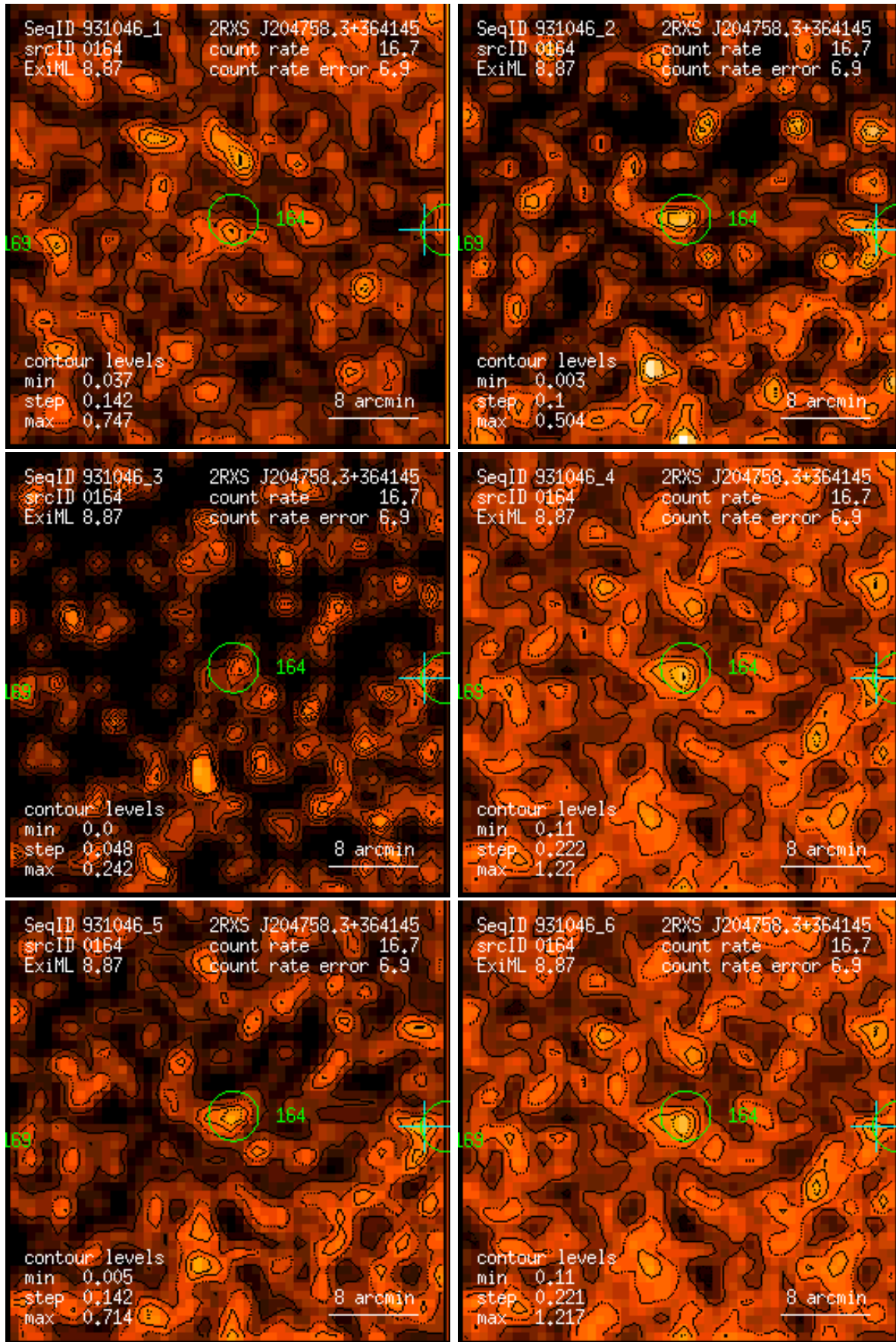
Figure 164: RASS 931046: detection 0164: band rate images, Gaussian filter: (1) PSPC channels 11 – 41, (2) 52 – 90, (3) 91 – 201, (4) 11 – 235, (5) 52 – 201, (6) 11 – 201. Broad band rates in counts/ks. Band rate contour levels in counts/ks/arcmin 2 .
