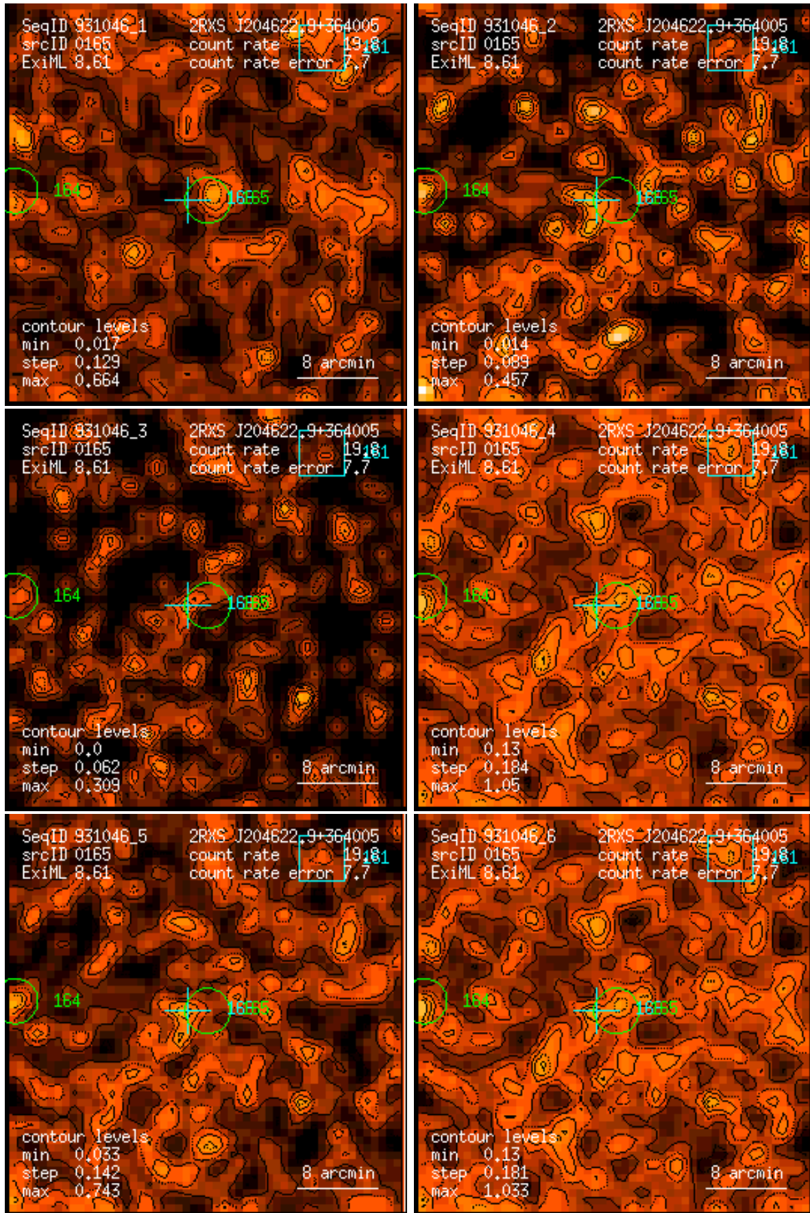
Figure 165: RASS 931046: detection 0165: band rate images, Gaussian filter: (1) PSPC channels 11 – 41, (2) 52 – 90, (3) 91 – 201, (4) 11 – 235, (5) 52 – 201, (6) 11 – 201. Broad band rates in counts/ks. Band rate contour levels in counts/ks/arcmin 2 .
