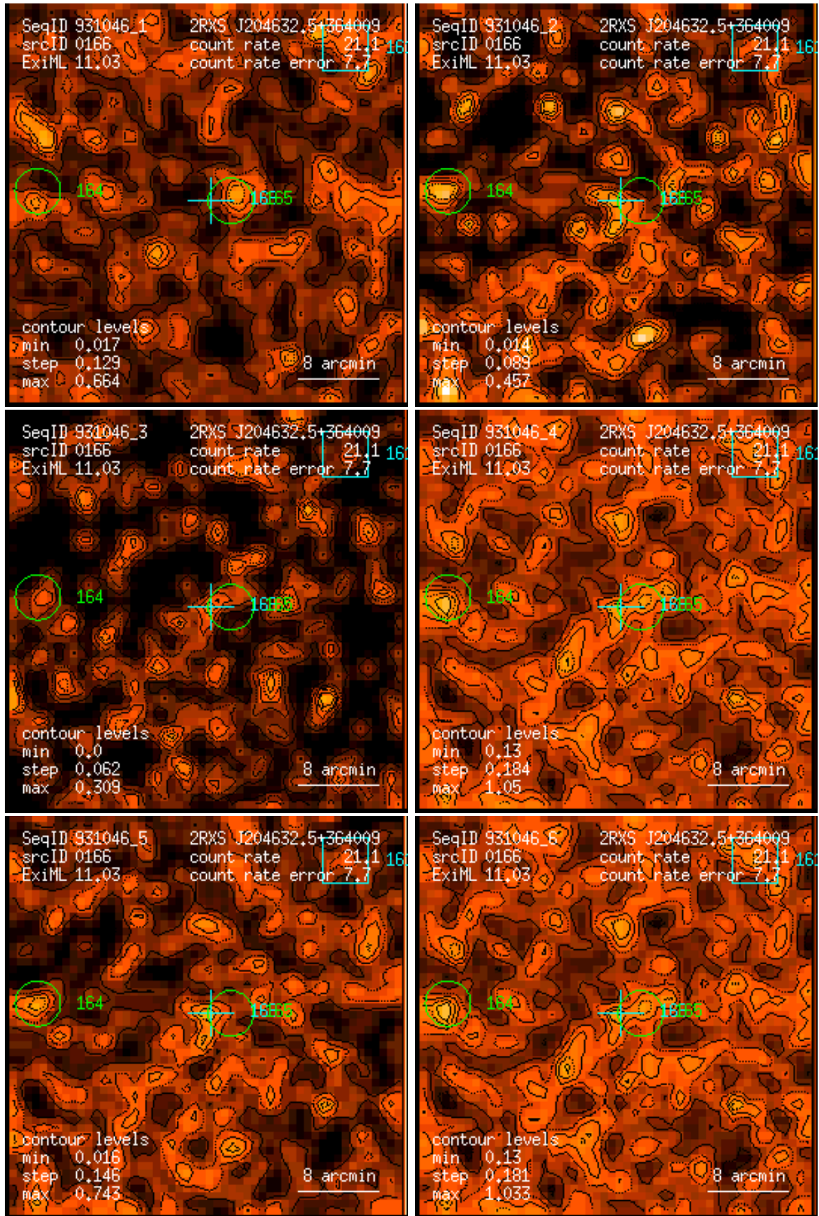
Figure 166: RASS 931046: detection 0166: band rate images, Gaussian filter: (1) PSPC channels 11 – 41, (2) 52 – 90, (3) 91 – 201, (4) 11 – 235, (5) 52 – 201, (6) 11 – 201. Broad band rates in counts/ks. Band rate contour levels in counts/ks/arcmin 2 .
