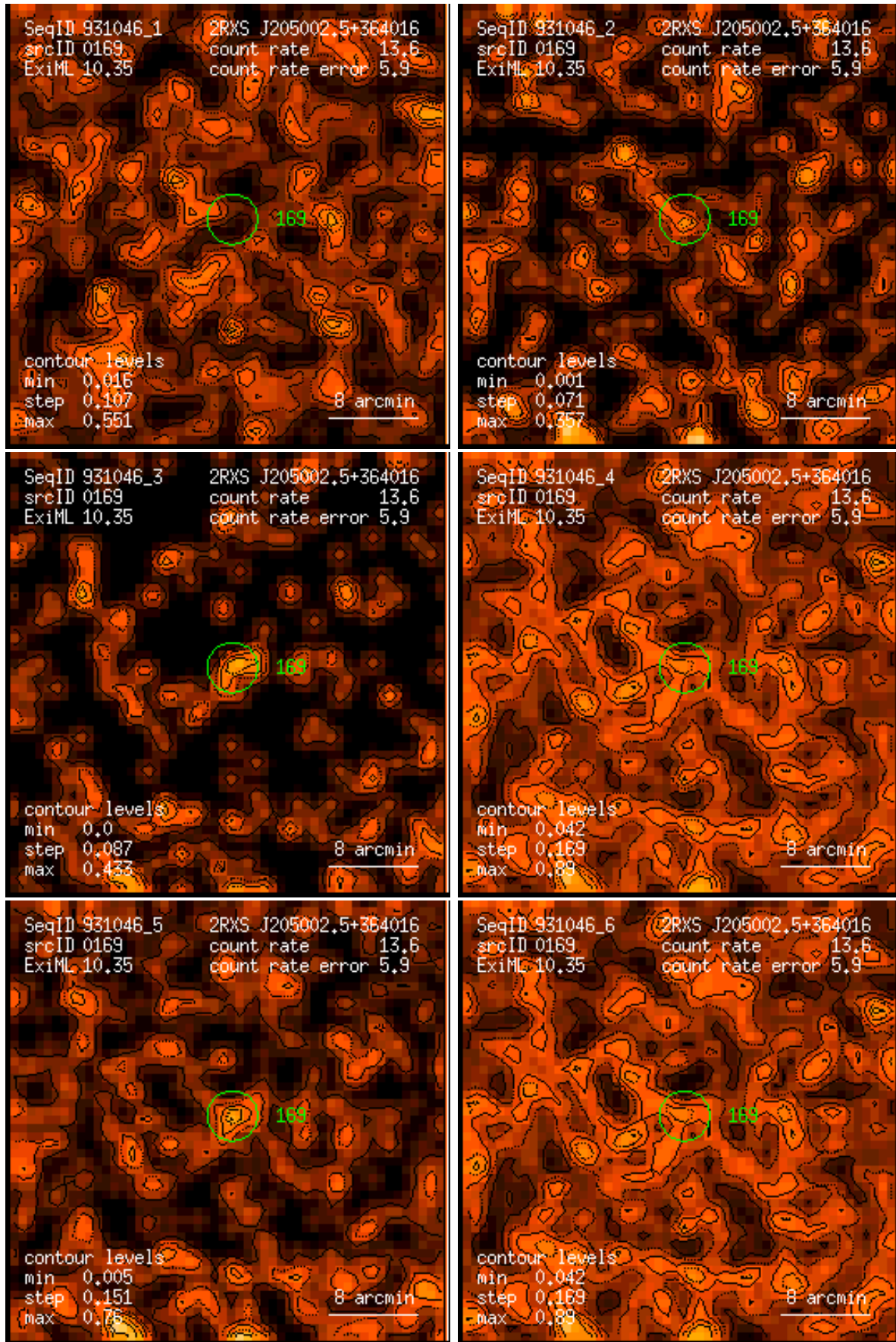
Figure 169: RASS 931046: detection 0169: band rate images, Gaussian filter: (1) PSPC channels 11 – 41, (2) 52 – 90, (3) 91 – 201, (4) 11 – 235, (5) 52 – 201, (6) 11 – 201. Broad band rates in counts/ks. Band rate contour levels in counts/ks/arcmin 2 .
