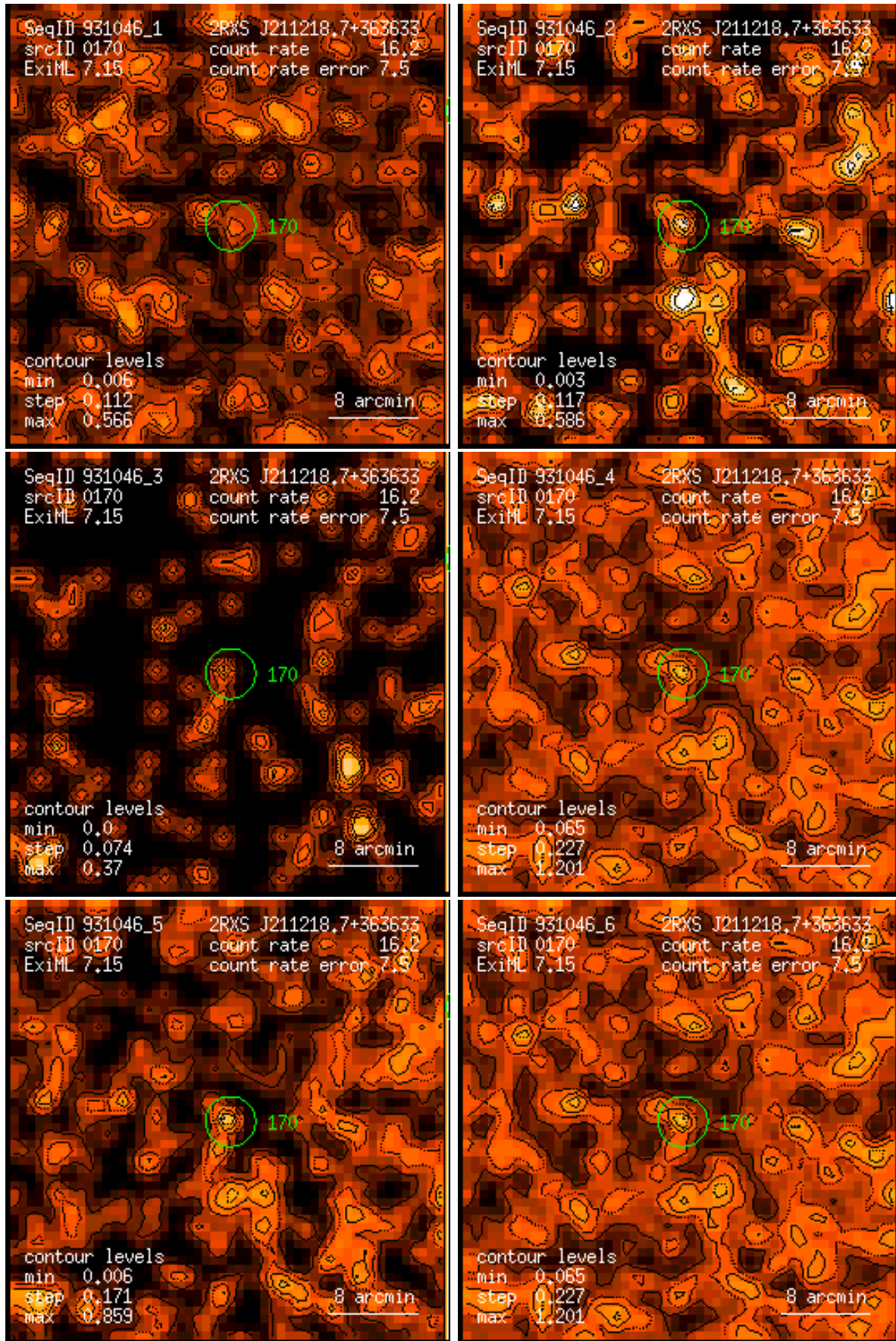
Figure 170: RASS 931046: detection 0170: band rate images, Gaussian filter: (1) PSPC channels 11 – 41, (2) 52 – 90, (3) 91 – 201, (4) 11 – 235, (5) 52 – 201, (6) 11 – 201. Broad band rates in counts/ks. Band rate contour levels in counts/ks/arcmin 2 .
