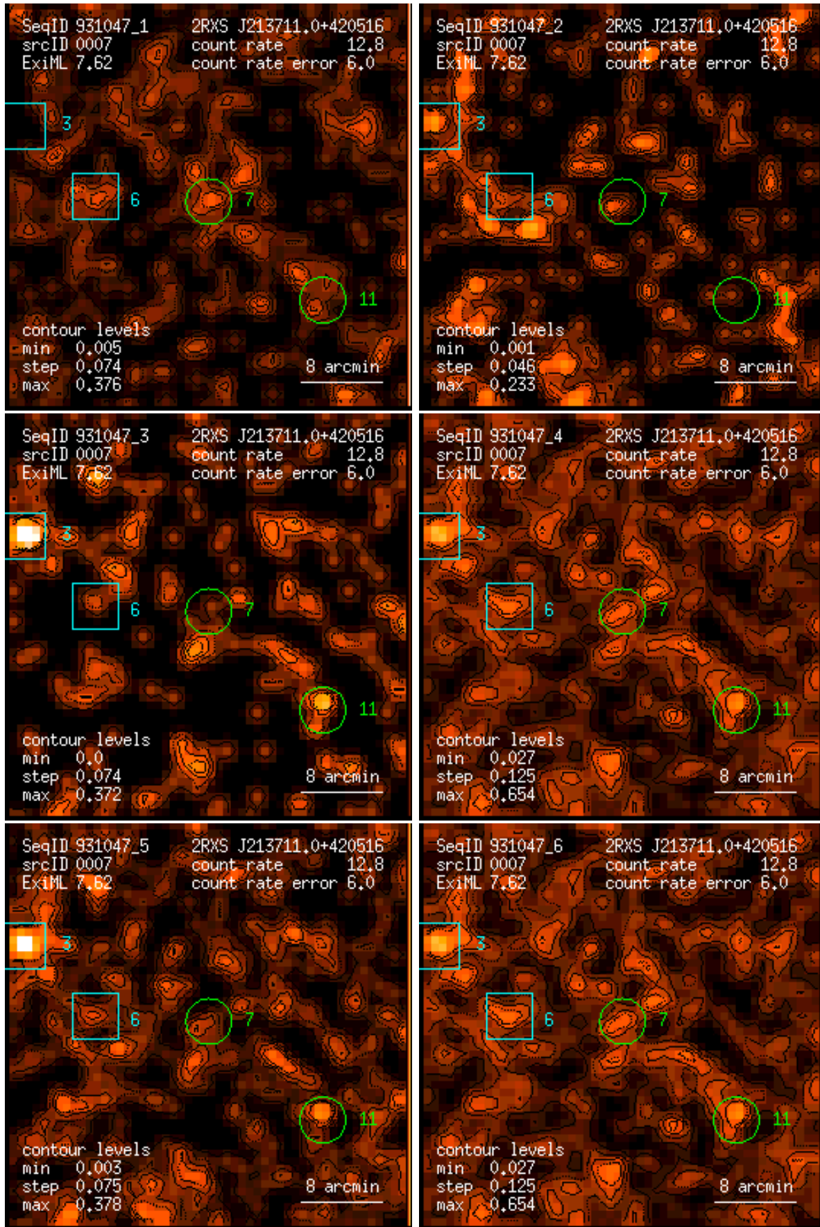
Figure 7: RASS 931047: detection 0007: band rate images, Gaussian filter: (1) PSPC channels 11 – 41, (2) 52 – 90, (3) 91 – 201, (4) 11 – 235, (5) 52 – 201, (6) 11 – 201. Broad band rates in counts/ks. Band rate contour levels in counts/ks/arcmin 2 .
