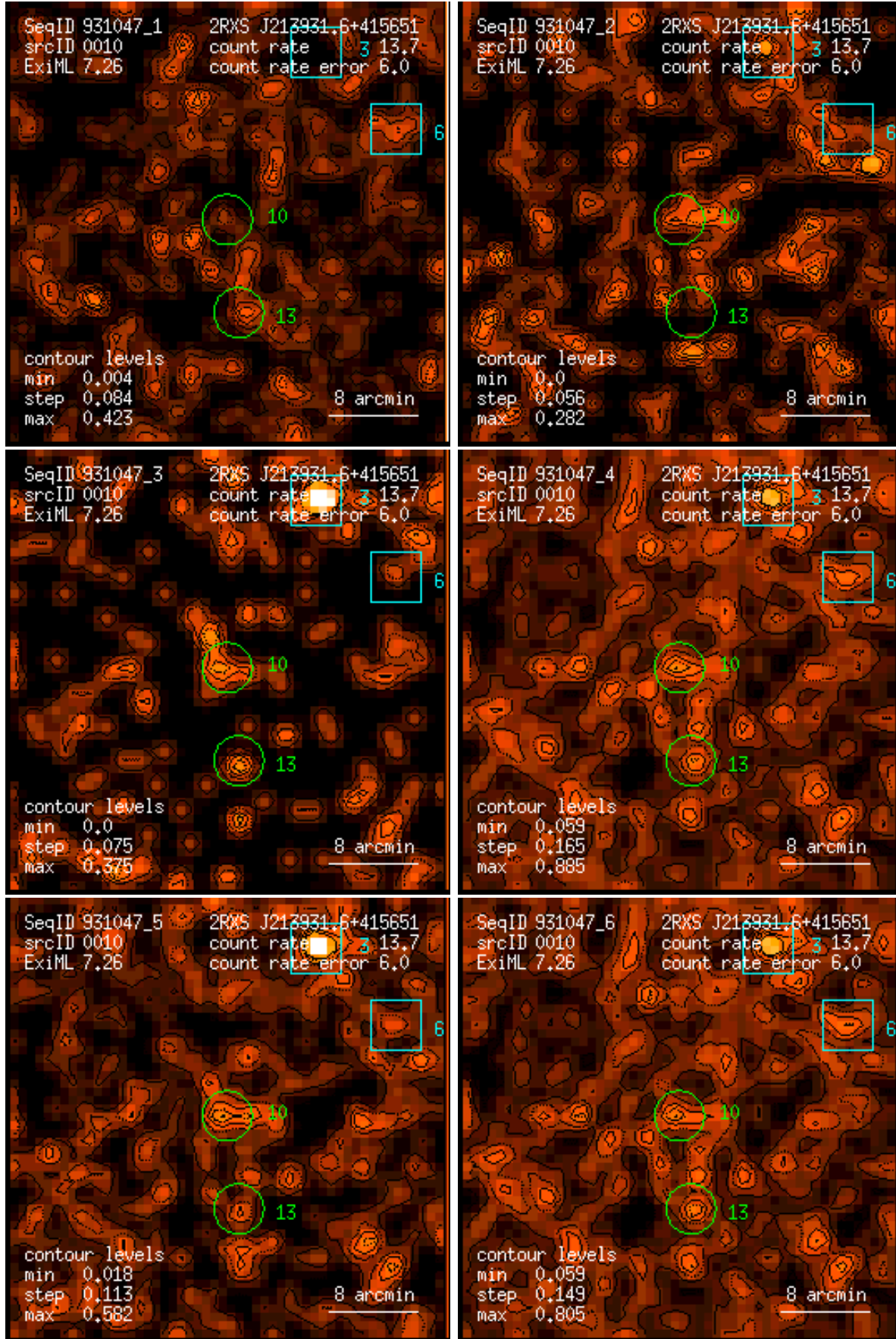
Figure 10: RASS 931047: detection 0010: band rate images, Gaussian filter: (1) PSPC channels 11 – 41, (2) 52 – 90, (3) 91 – 201, (4) 11 – 235, (5) 52 – 201, (6) 11 – 201. Broad band rates in counts/ks. Band rate contour levels in counts/ks/arcmin 2 .
