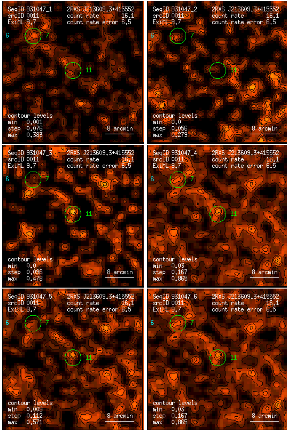
Figure 11: RASS 931047: detection 0011: band rate images, Gaussian filter: (1) PSPC channels 11 – 41, (2) 52 – 90, (3) 91 – 201, (4) 11 – 235, (5) 52 – 201, (6) 11 – 201. Broad band rates in counts/ks. Band rate contour levels in counts/ks/arcmin 2 .
