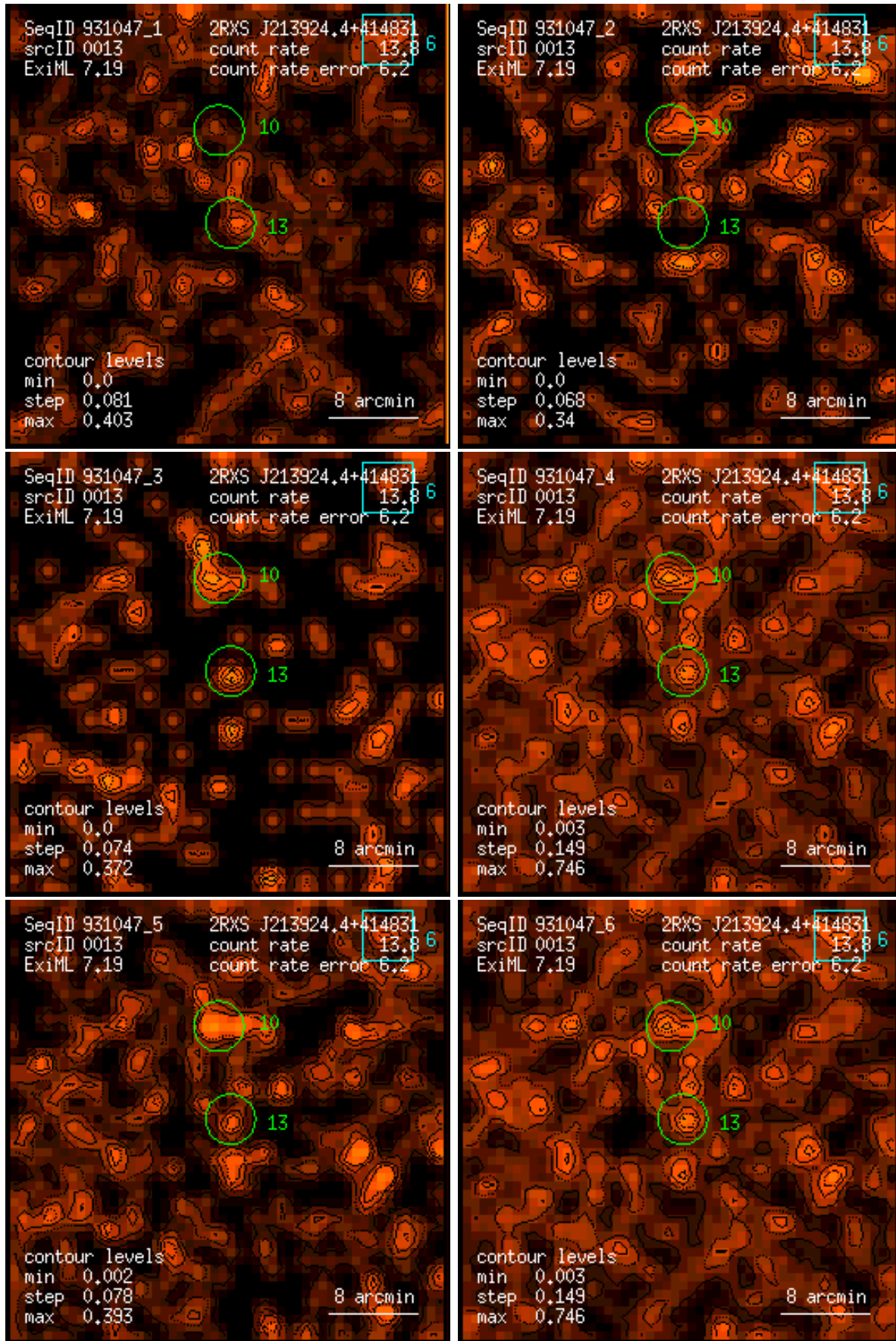
Figure 13: RASS 931047: detection 0013: band rate images, Gaussian filter: (1) PSPC channels 11 – 41, (2) 52 – 90, (3) 91 – 201, (4) 11 – 235, (5) 52 – 201, (6) 11 – 201. Broad band rates in counts/ks. Band rate contour levels in counts/ks/arcmin 2 .
