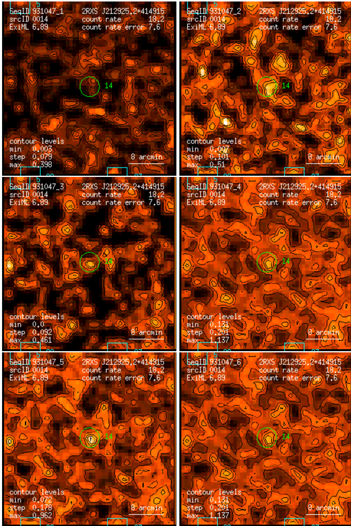
Figure 14: RASS 931047: detection 0014: band rate images, Gaussian filter: (1) PSPC channels 11 – 41, (2) 52 – 90, (3) 91 – 201, (4) 11 – 235, (5) 52 – 201, (6) 11 – 201. Broad band rates in counts/ks. Band rate contour levels in counts/ks/arcmin 2 .
