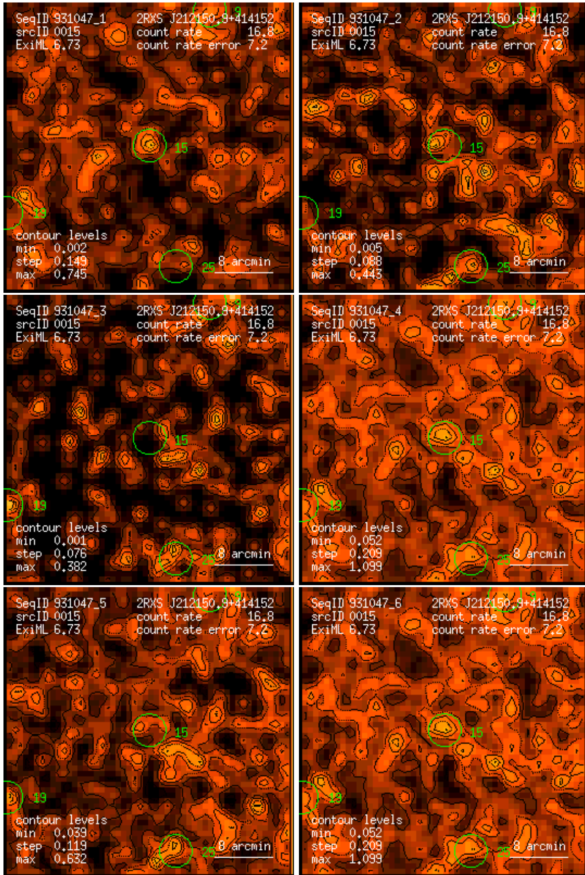
Figure 15: RASS 931047: detection 0015: band rate images, Gaussian filter: (1) PSPC channels 11 – 41, (2) 52 – 90, (3) 91 – 201, (4) 11 – 235, (5) 52 – 201, (6) 11 – 201. Broad band rates in counts/ks. Band rate contour levels in counts/ks/arcmin 2 .
