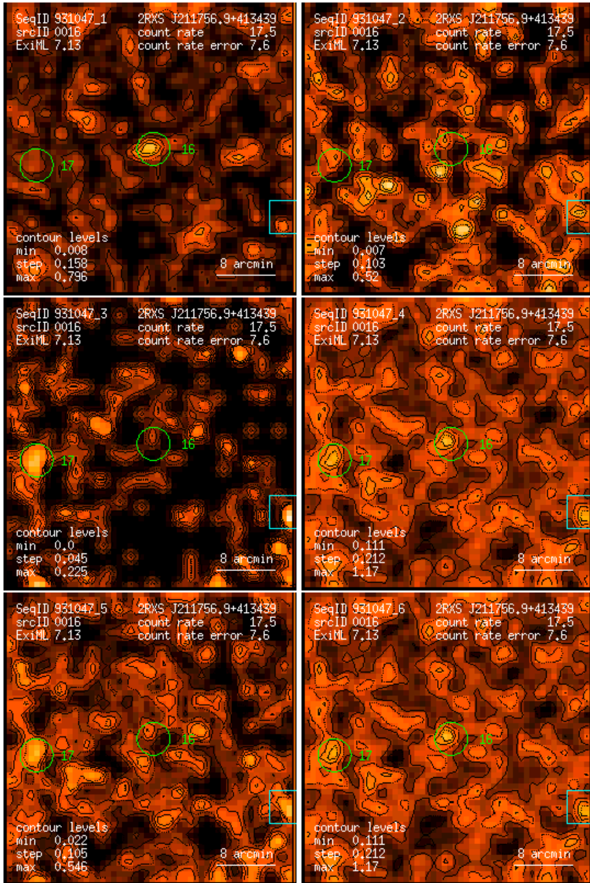
Figure 16: RASS 931047: detection 0016: band rate images, Gaussian filter: (1) PSPC channels 11 – 41, (2) 52 – 90, (3) 91 – 201, (4) 11 – 235, (5) 52 – 201, (6) 11 – 201. Broad band rates in counts/ks. Band rate contour levels in counts/ks/arcmin 2 .
