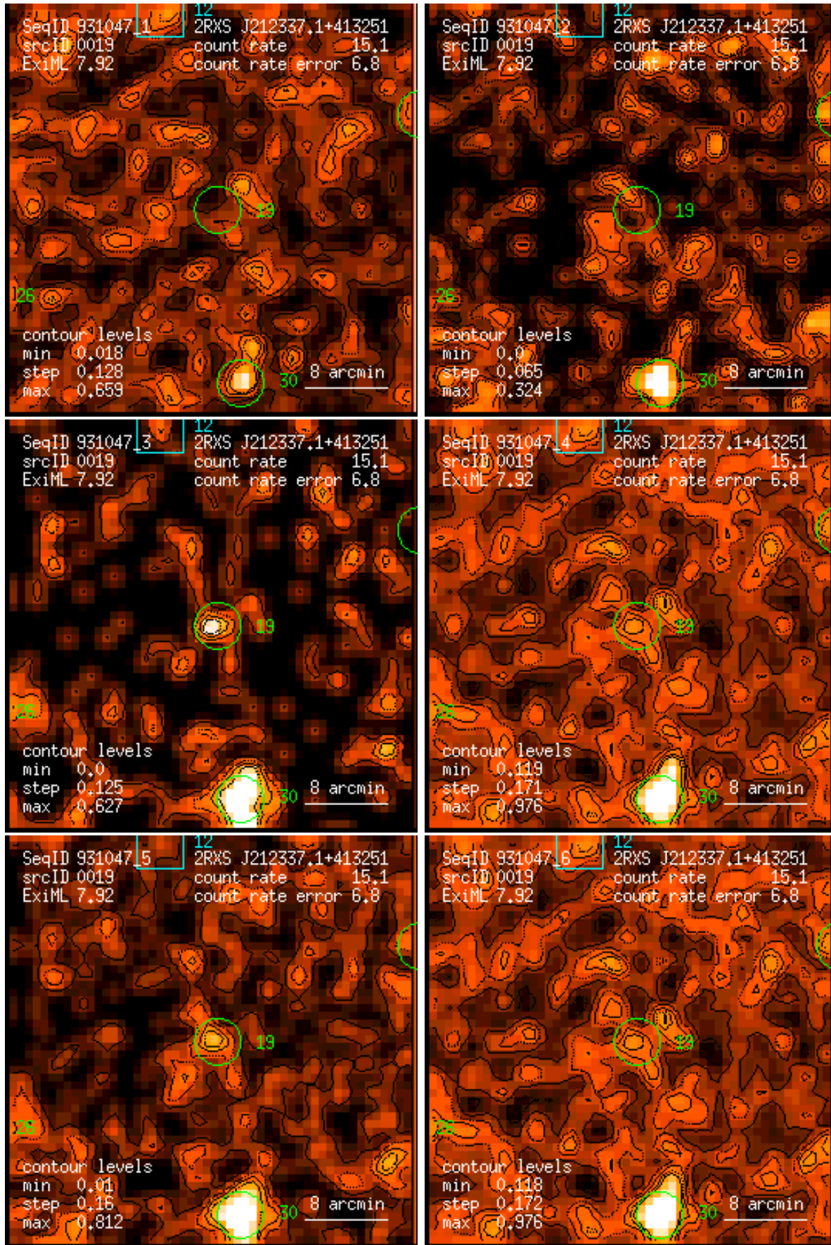
Figure 19: RASS 931047: detection 0019: band rate images, Gaussian filter: (1) PSPC channels 11 – 41, (2) 52 – 90, (3) 91 – 201, (4) 11 – 235, (5) 52 – 201, (6) 11 – 201. Broad band rates in counts/ks. Band rate contour levels in counts/ks/arcmin 2 .
