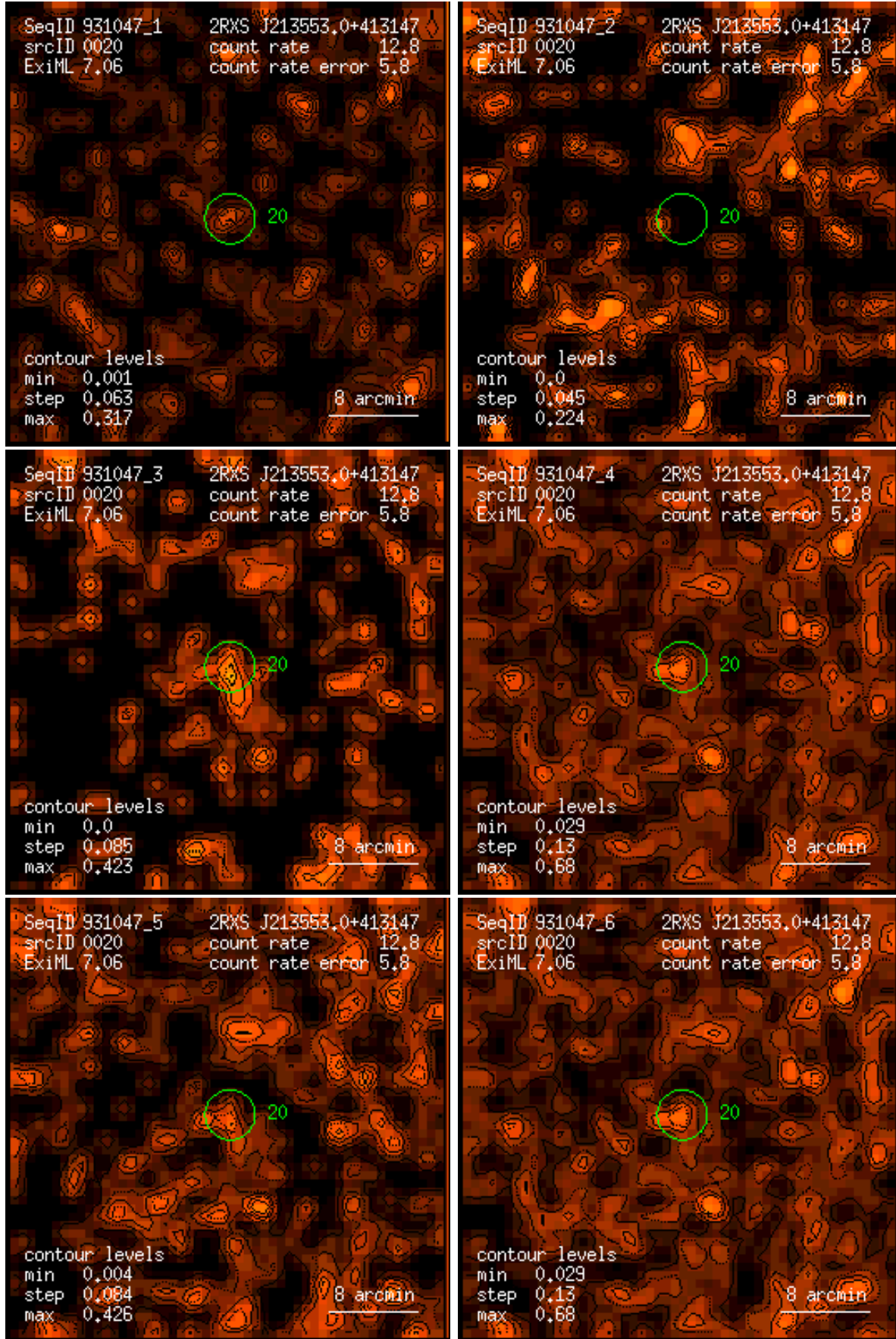
Figure 20: RASS 931047: detection 0020: band rate images, Gaussian filter: (1) PSPC channels 11 – 41, (2) 52 – 90, (3) 91 – 201, (4) 11 – 235, (5) 52 – 201, (6) 11 – 201. Broad band rates in counts/ks. Band rate contour levels in counts/ks/arcmin 2 .
