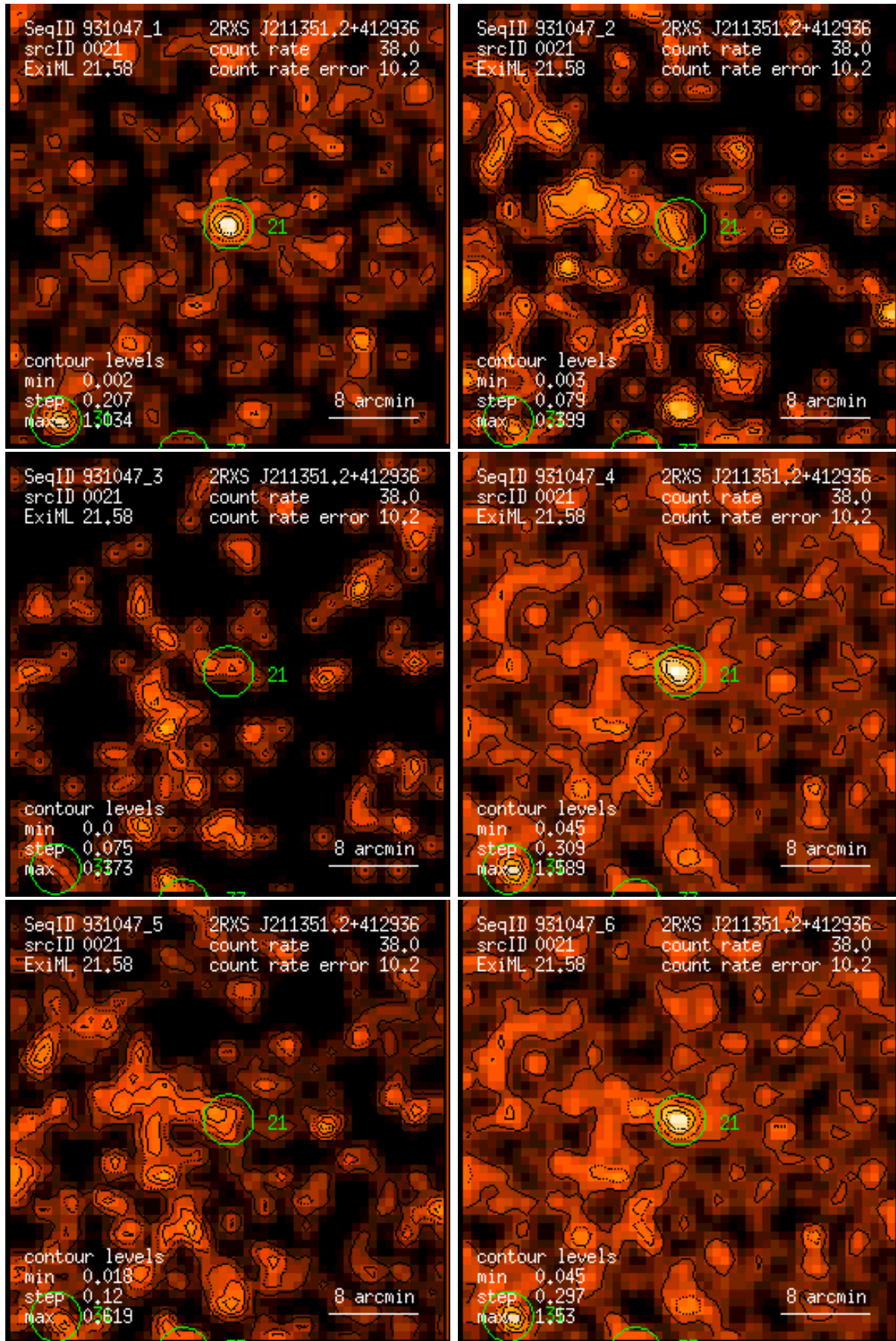
Figure 21: RASS 931047: detection 0021: band rate images, Gaussian filter: (1) PSPC channels 11 – 41, (2) 52 – 90, (3) 91 – 201, (4) 11 – 235, (5) 52 – 201, (6) 11 – 201. Broad band rates in counts/ks. Band rate contour levels in counts/ks/arcmin 2 .
