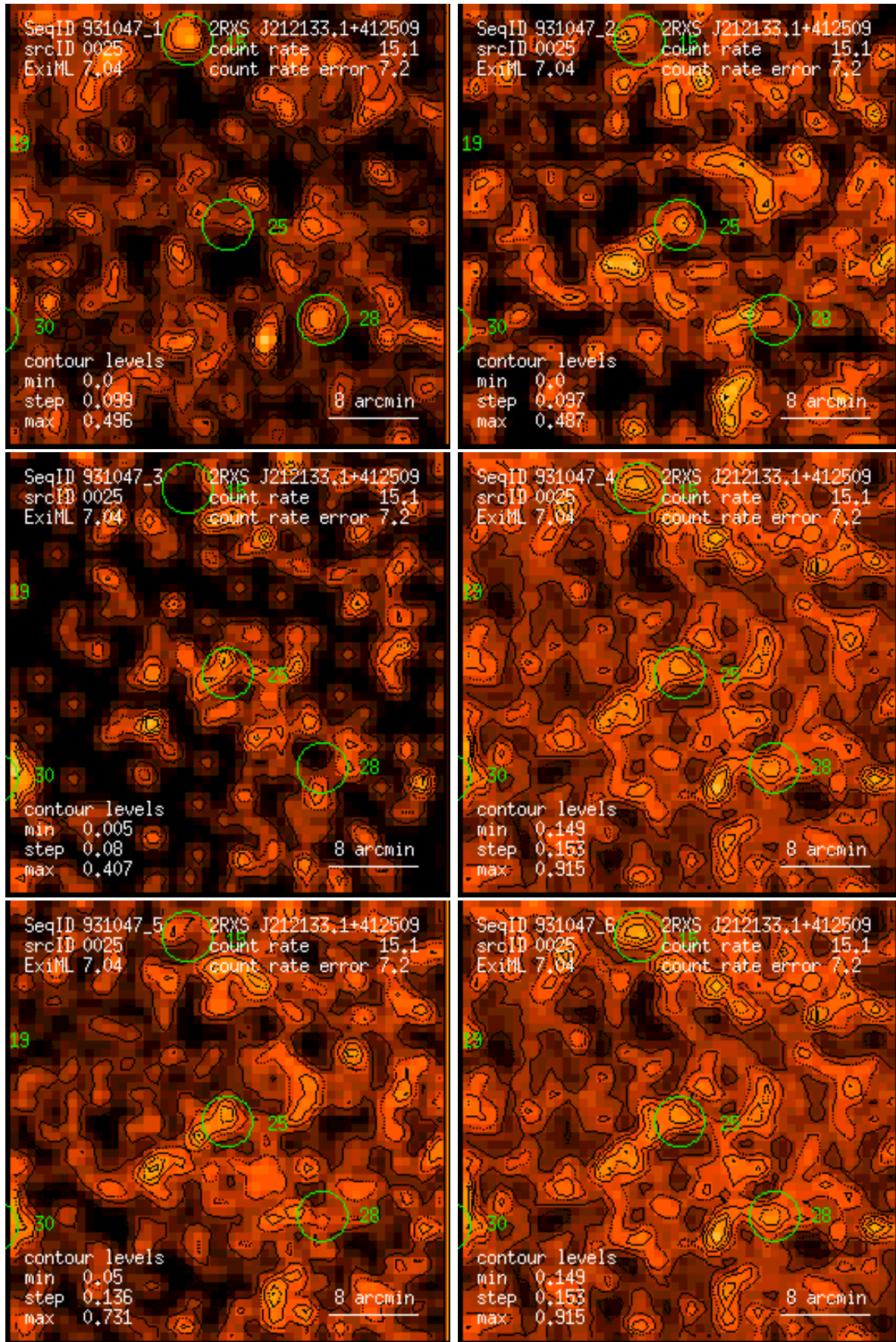
Figure 25: RASS 931047: detection 0025: band rate images, Gaussian filter: (1) PSPC channels 11 – 41, (2) 52 – 90, (3) 91 – 201, (4) 11 – 235, (5) 52 – 201, (6) 11 – 201. Broad band rates in counts/ks. Band rate contour levels in counts/ks/arcmin 2 .
