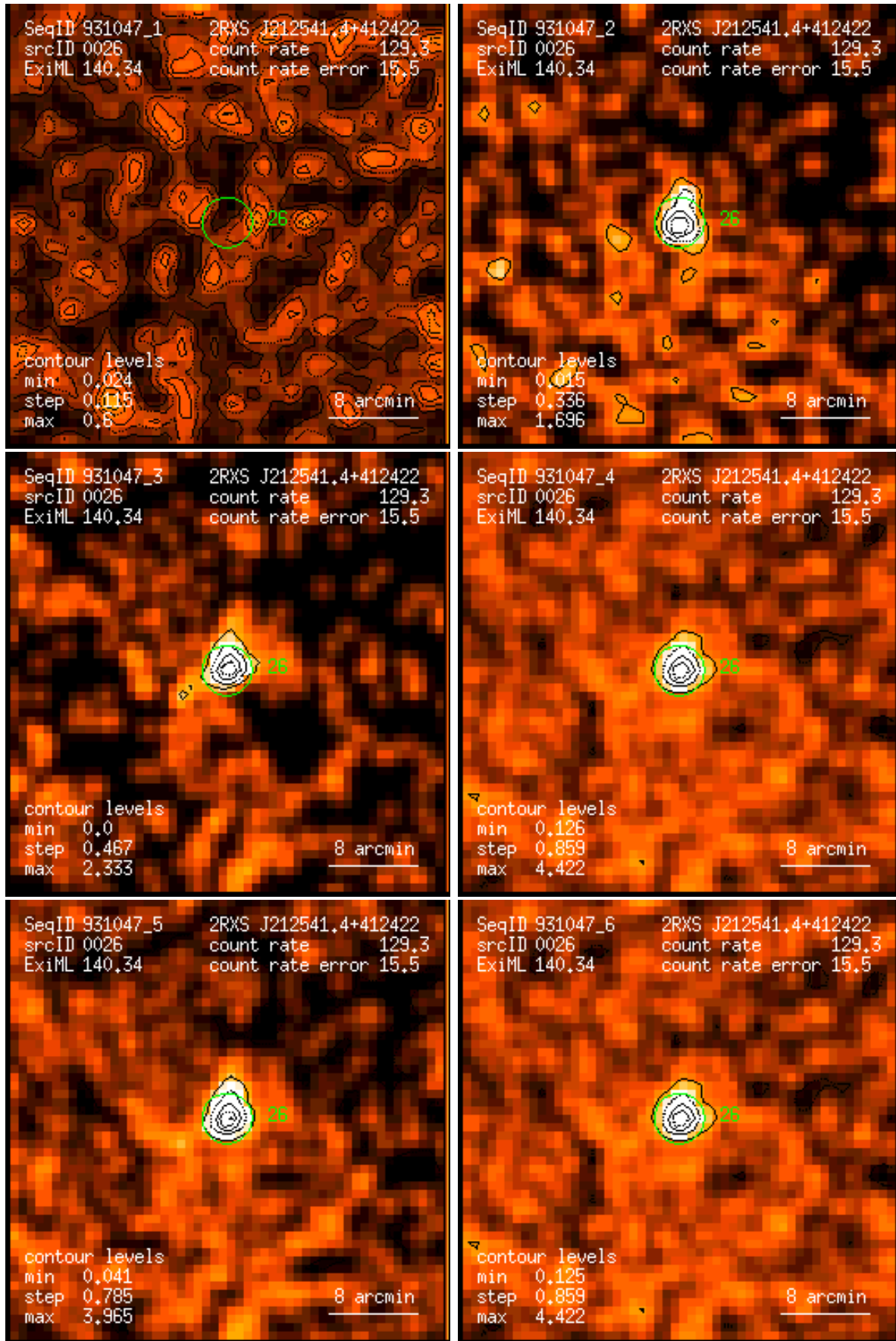
Figure 26: RASS 931047: detection 0026: band rate images, Gaussian filter: (1) PSPC channels 11 – 41, (2) 52 – 90, (3) 91 – 201, (4) 11 – 235, (5) 52 – 201, (6) 11 – 201. Broad band rates in counts/ks. Band rate contour levels in counts/ks/arcmin 2 .
