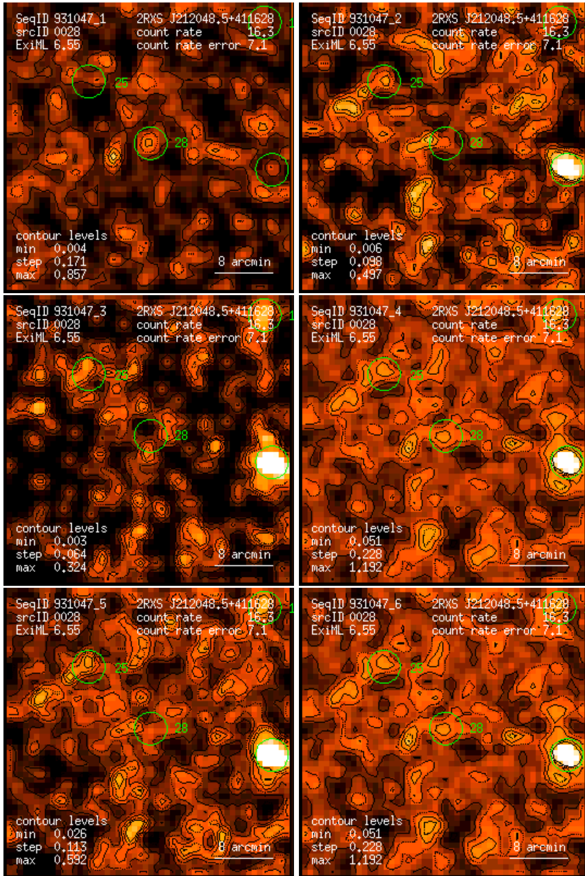
Figure 28: RASS 931047: detection 0028: band rate images, Gaussian filter: (1) PSPC channels 11 – 41, (2) 52 – 90, (3) 91 – 201, (4) 11 – 235, (5) 52 – 201, (6) 11 – 201. Broad band rates in counts/ks. Band rate contour levels in counts/ks/arcmin 2 .
