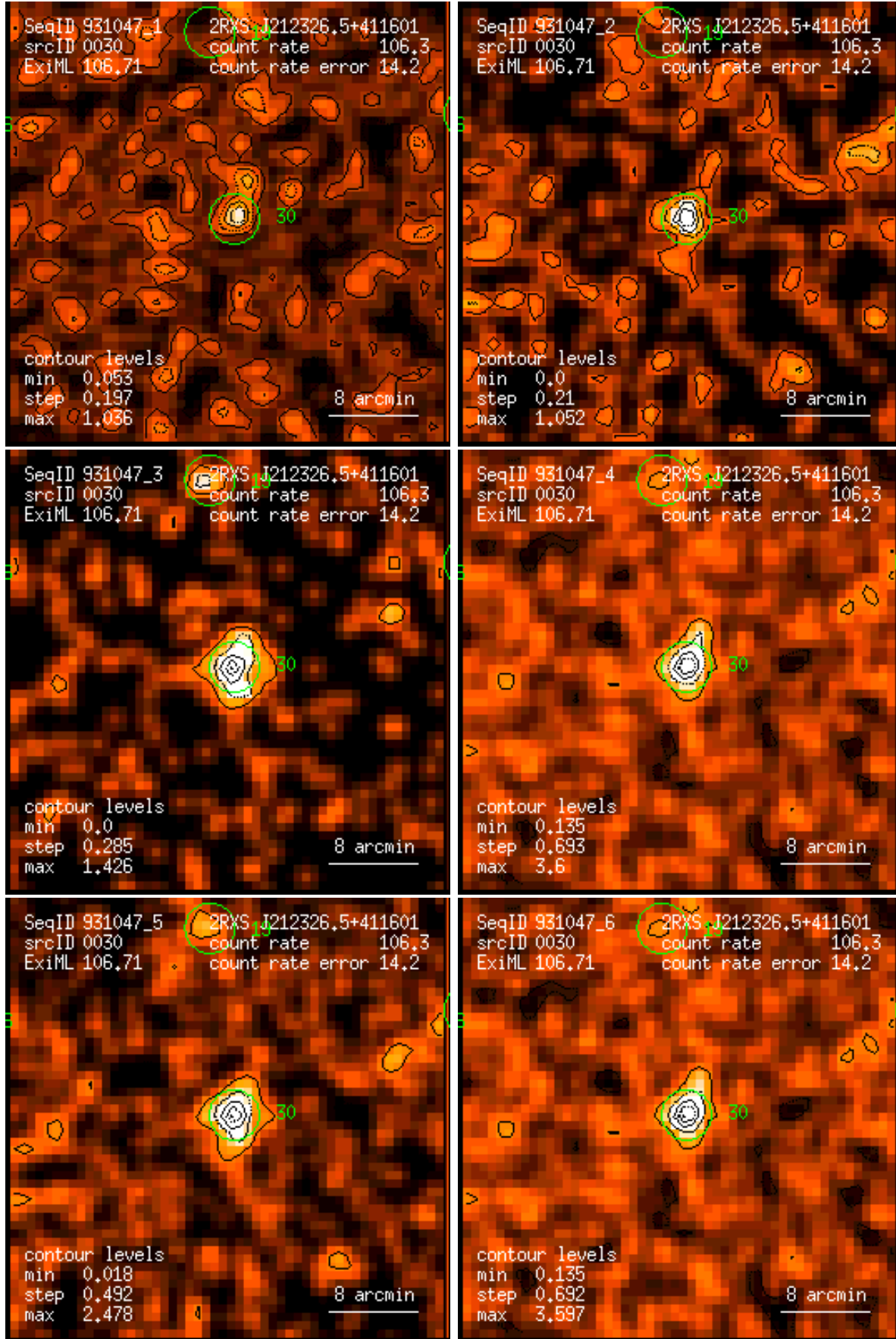
Figure 30: RASS 931047: detection 0030: band rate images, Gaussian filter: (1) PSPC channels 11 – 41, (2) 52 – 90, (3) 91 – 201, (4) 11 – 235, (5) 52 – 201, (6) 11 – 201. Broad band rates in counts/ks. Band rate contour levels in counts/ks/arcmin 2 .
