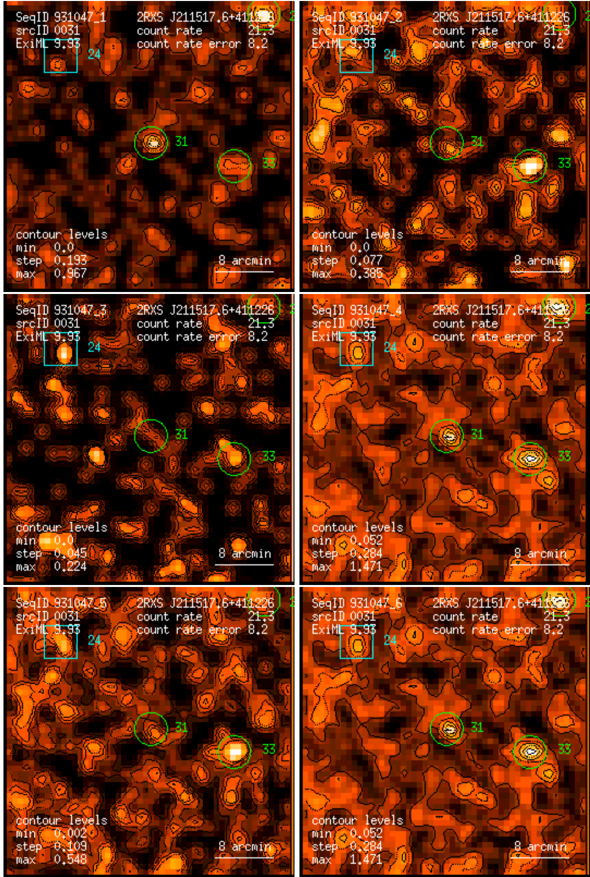
Figure 31: RASS 931047: detection 0031: band rate images, Gaussian filter: (1) PSPC channels 11 – 41, (2) 52 – 90, (3) 91 – 201, (4) 11 – 235, (5) 52 – 201, (6) 11 – 201. Broad band rates in counts/ks. Band rate contour levels in counts/ks/arcmin 2 .
