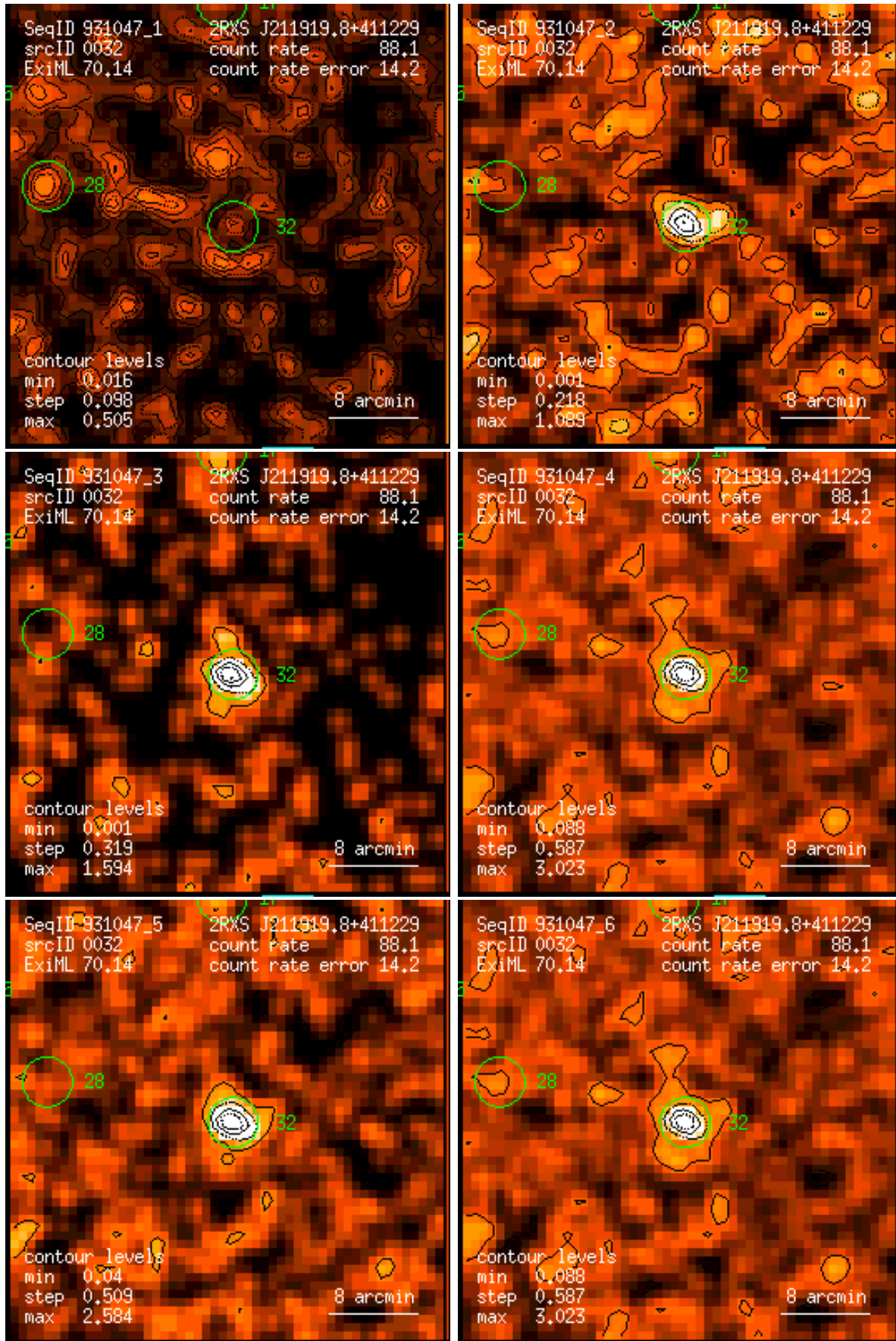
Figure 32: RASS 931047: detection 0032: band rate images, Gaussian filter: (1) PSPC channels 11 – 41, (2) 52 – 90, (3) 91 – 201, (4) 11 – 235, (5) 52 – 201, (6) 11 – 201. Broad band rates in counts/ks. Band rate contour levels in counts/ks/arcmin 2 .
