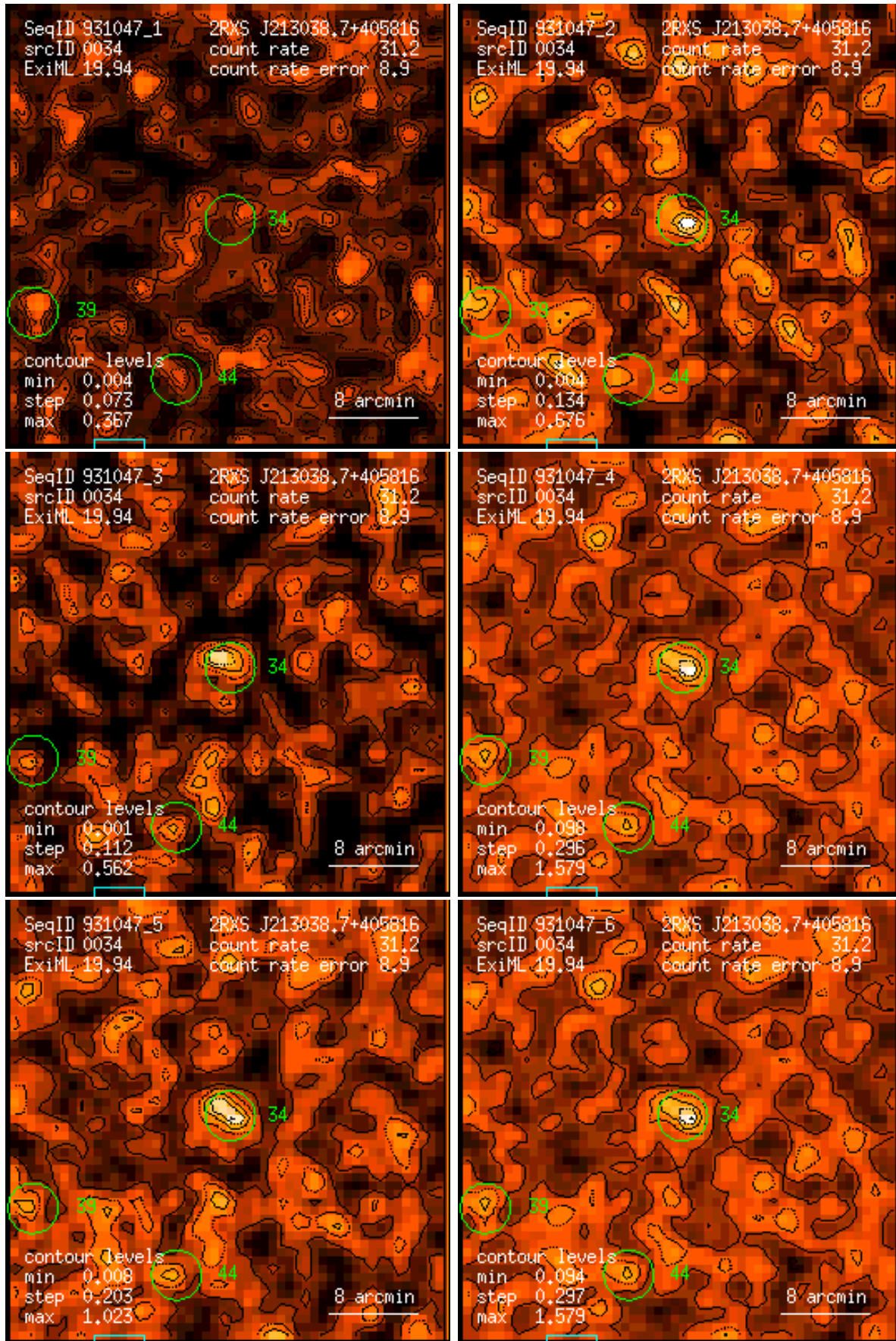
Figure 34: RASS 931047: detection 0034: band rate images, Gaussian filter: (1) PSPC channels 11 – 41, (2) 52 – 90, (3) 91 – 201, (4) 11 – 235, (5) 52 – 201, (6) 11 – 201. Broad band rates in counts/ks. Band rate contour levels in counts/ks/arcmin 2 .
