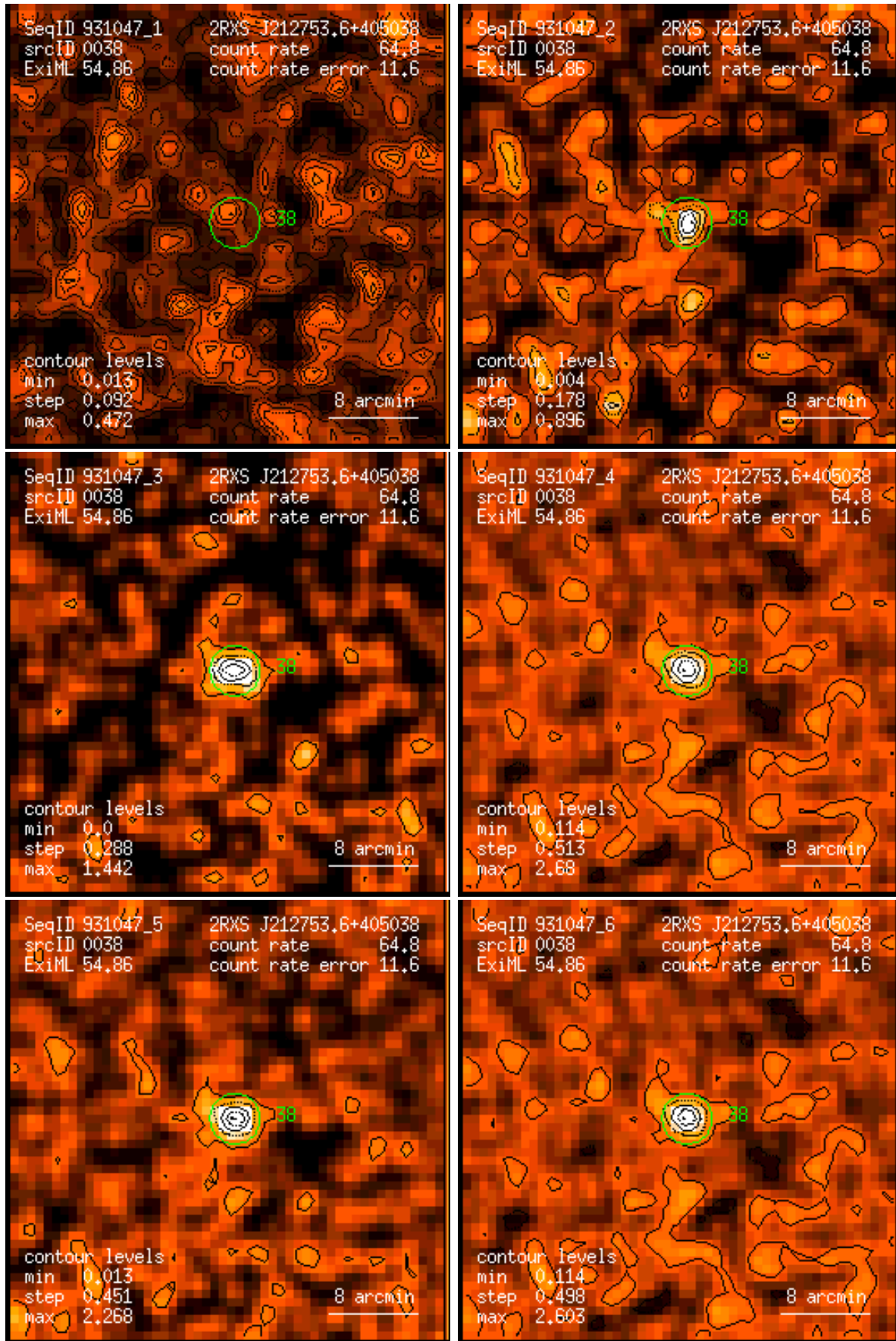
Figure 38: RASS 931047: detection 0038: band rate images, Gaussian filter: (1) PSPC channels 11 – 41, (2) 52 – 90, (3) 91 – 201, (4) 11 – 235, (5) 52 – 201, (6) 11 – 201. Broad band rates in counts/ks. Band rate contour levels in counts/ks/arcmin 2 .
