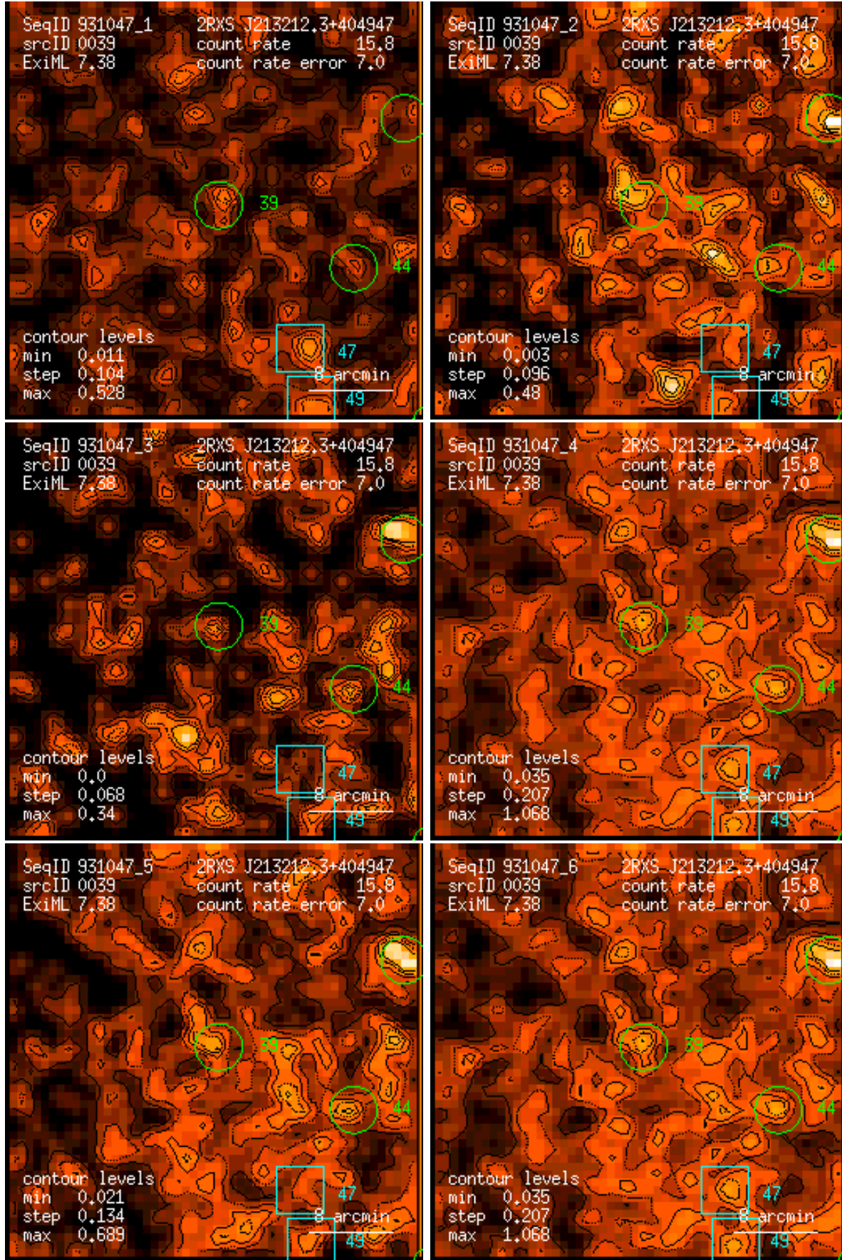
Figure 39: RASS 931047: detection 0039: band rate images, Gaussian filter: (1) PSPC channels 11 – 41, (2) 52 – 90, (3) 91 – 201, (4) 11 – 235, (5) 52 – 201, (6) 11 – 201. Broad band rates in counts/ks. Band rate contour levels in counts/ks/arcmin 2 .
