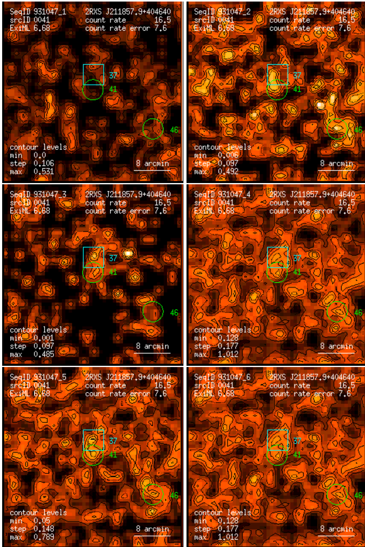
Figure 41: RASS 931047: detection 0041: band rate images, Gaussian filter: (1) PSPC channels 11 – 41, (2) 52 – 90, (3) 91 – 201, (4) 11 – 235, (5) 52 – 201, (6) 11 – 201. Broad band rates in counts/ks. Band rate contour levels in counts/ks/arcmin 2 .
