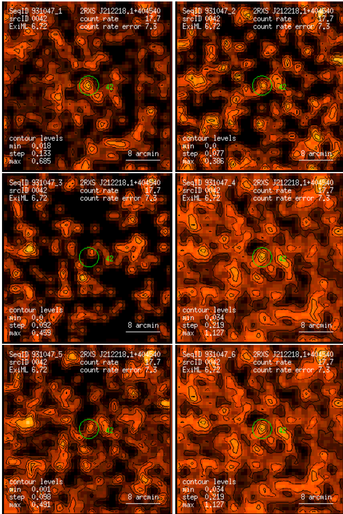
Figure 42: RASS 931047: detection 0042: band rate images, Gaussian filter: (1) PSPC channels 11 – 41, (2) 52 – 90, (3) 91 – 201, (4) 11 – 235, (5) 52 – 201, (6) 11 – 201. Broad band rates in counts/ks. Band rate contour levels in counts/ks/arcmin 2 .
