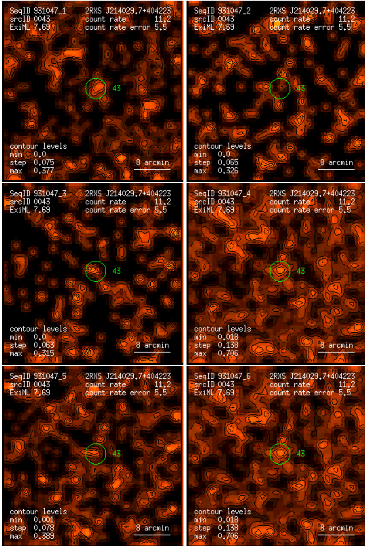
Figure 43: RASS 931047: detection 0043: band rate images, Gaussian filter: (1) PSPC channels 11 – 41, (2) 52 – 90, (3) 91 – 201, (4) 11 – 235, (5) 52 – 201, (6) 11 – 201. Broad band rates in counts/ks. Band rate contour levels in counts/ks/arcmin 2 .
