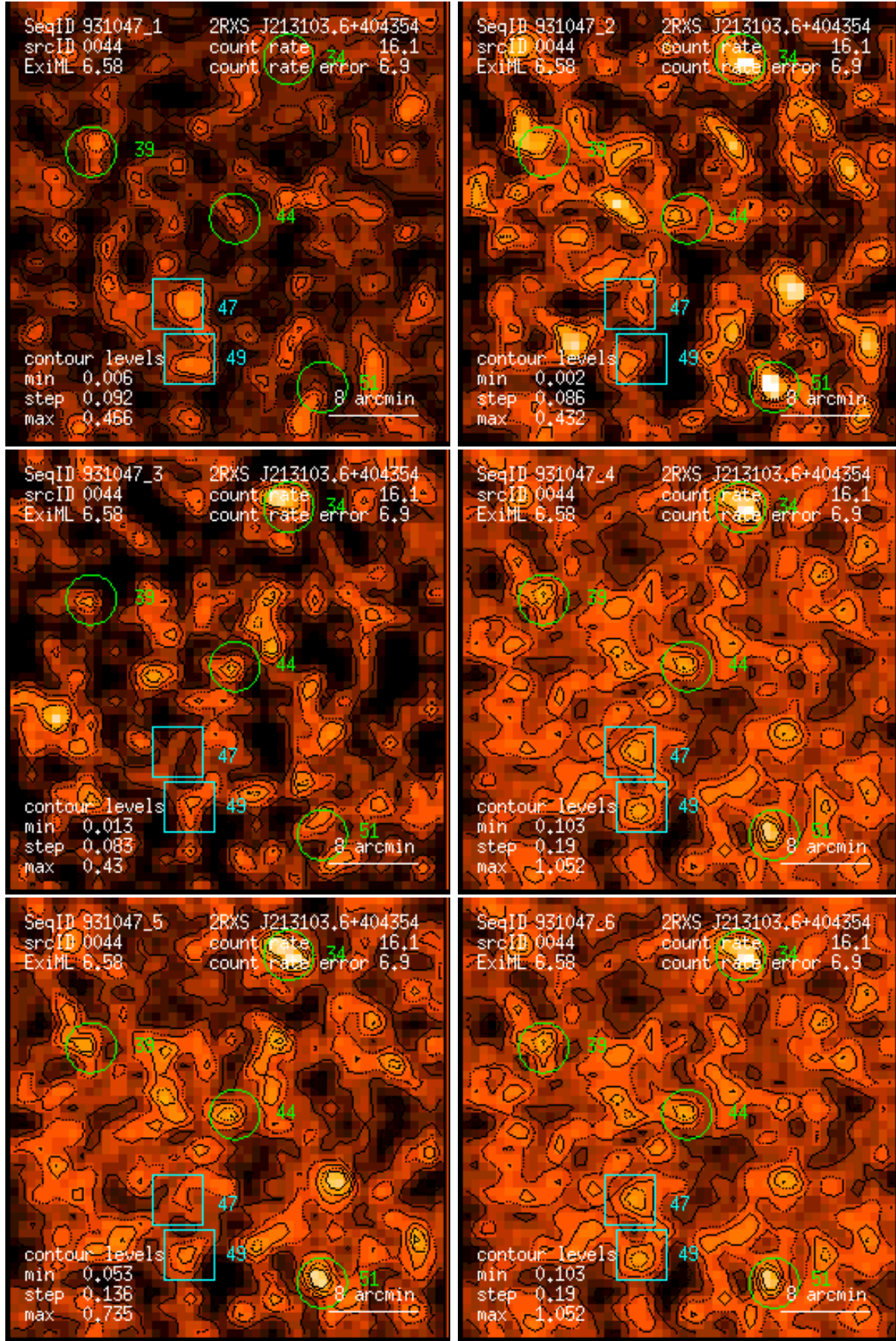
Figure 44: RASS 931047: detection 0044: band rate images, Gaussian filter: (1) PSPC channels 11 – 41, (2) 52 – 90, (3) 91 – 201, (4) 11 – 235, (5) 52 – 201, (6) 11 – 201. Broad band rates in counts/ks. Band rate contour levels in counts/ks/arcmin 2 .
