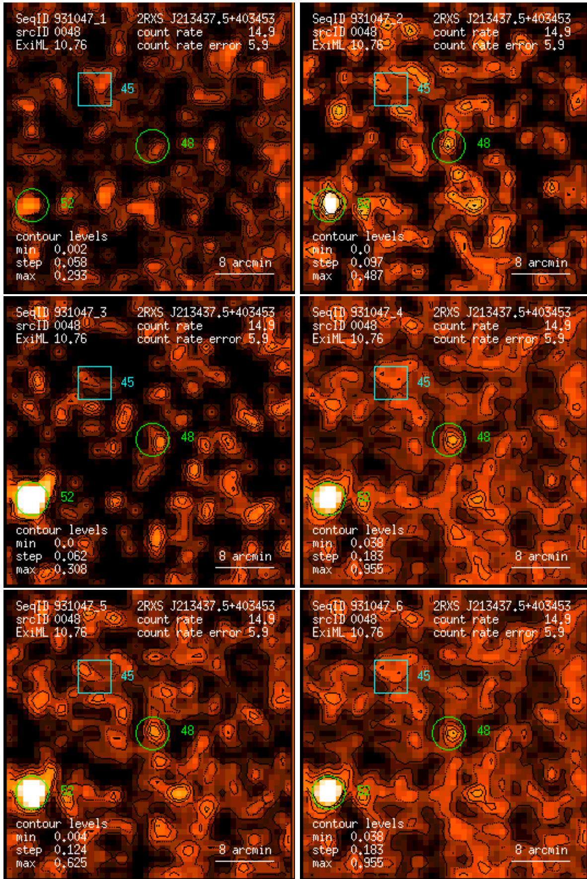
Figure 48: RASS 931047: detection 0048: band rate images, Gaussian filter: (1) PSPC channels 11 – 41, (2) 52 – 90, (3) 91 – 201, (4) 11 – 235, (5) 52 – 201, (6) 11 – 201. Broad band rates in counts/ks. Band rate contour levels in counts/ks/arcmin 2 .
