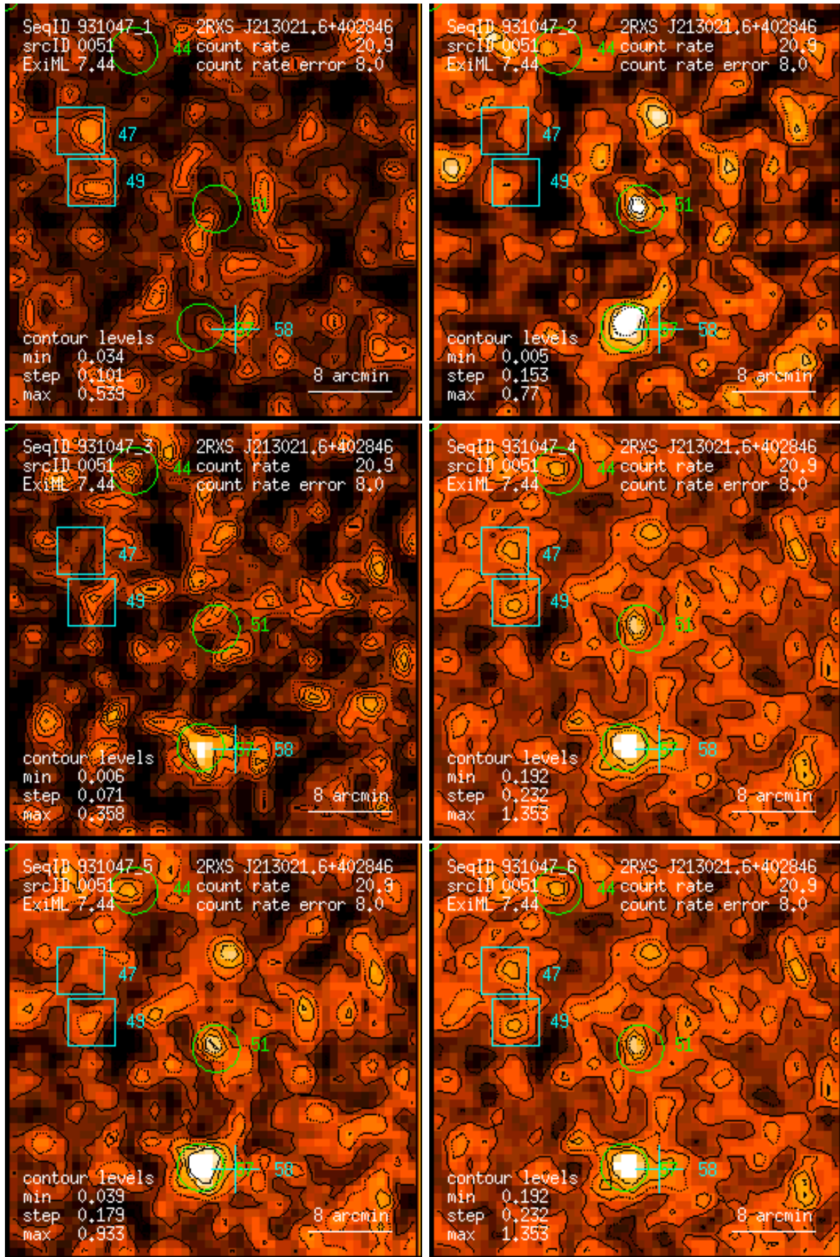
Figure 51: RASS 931047: detection 0051: band rate images, Gaussian filter: (1) PSPC channels 11 – 41, (2) 52 – 90, (3) 91 – 201, (4) 11 – 235, (5) 52 – 201, (6) 11 – 201. Broad band rates in counts/ks. Band rate contour levels in counts/ks/arcmin 2 .
