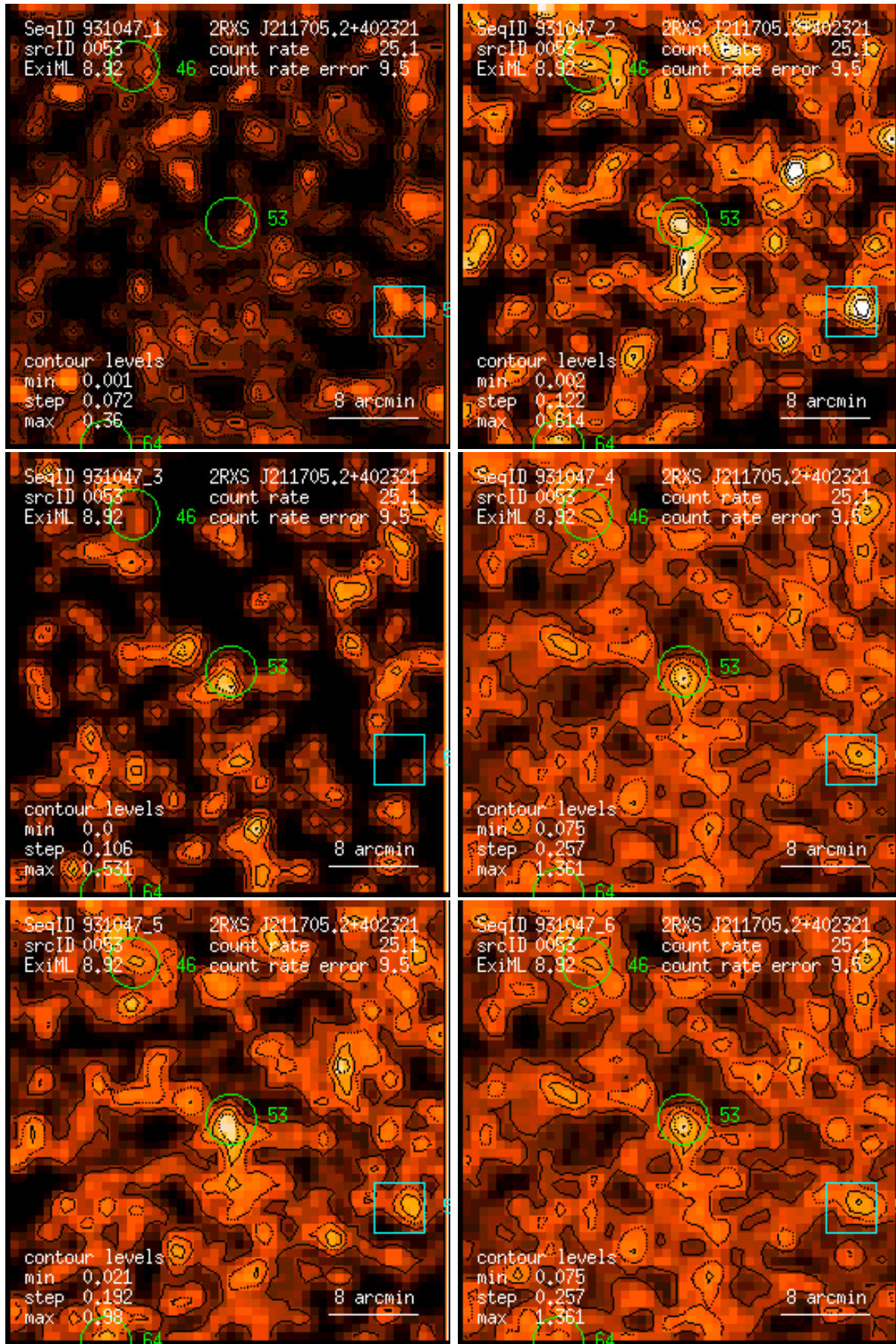
Figure 53: RASS 931047: detection 0053: band rate images, Gaussian filter: (1) PSPC channels 11 – 41, (2) 52 – 90, (3) 91 – 201, (4) 11 – 235, (5) 52 – 201, (6) 11 – 201. Broad band rates in counts/ks. Band rate contour levels in counts/ks/arcmin 2 .
