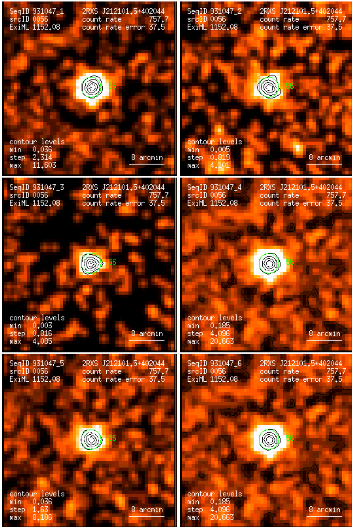
Figure 56: RASS 931047: detection 0056: band rate images, Gaussian filter: (1) PSPC channels 11 – 41, (2) 52 – 90, (3) 91 – 201, (4) 11 – 235, (5) 52 – 201, (6) 11 – 201. Broad band rates in counts/ks. Band rate contour levels in counts/ks/arcmin 2 .
