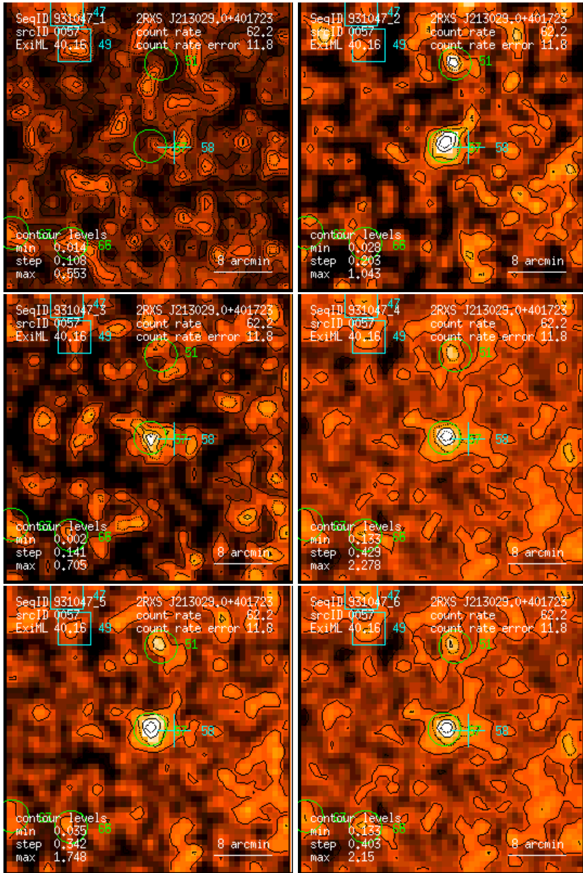
Figure 57: RASS 931047: detection 0057: band rate images, Gaussian filter: (1) PSPC channels 11 – 41, (2) 52 – 90, (3) 91 – 201, (4) 11 – 235, (5) 52 – 201, (6) 11 – 201. Broad band rates in counts/ks. Band rate contour levels in counts/ks/arcmin 2 .
