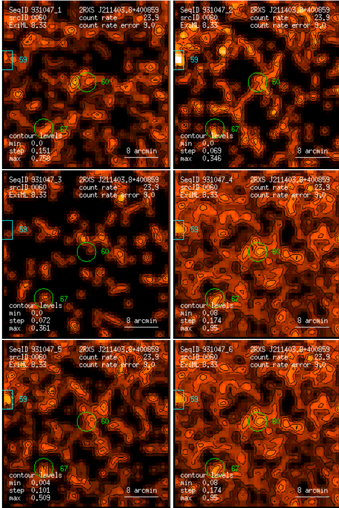
Figure 60: RASS 931047: detection 0060: band rate images, Gaussian filter: (1) PSPC channels 11 – 41, (2) 52 – 90, (3) 91 – 201, (4) 11 – 235, (5) 52 – 201, (6) 11 – 201. Broad band rates in counts/ks. Band rate contour levels in counts/ks/arcmin 2 .
