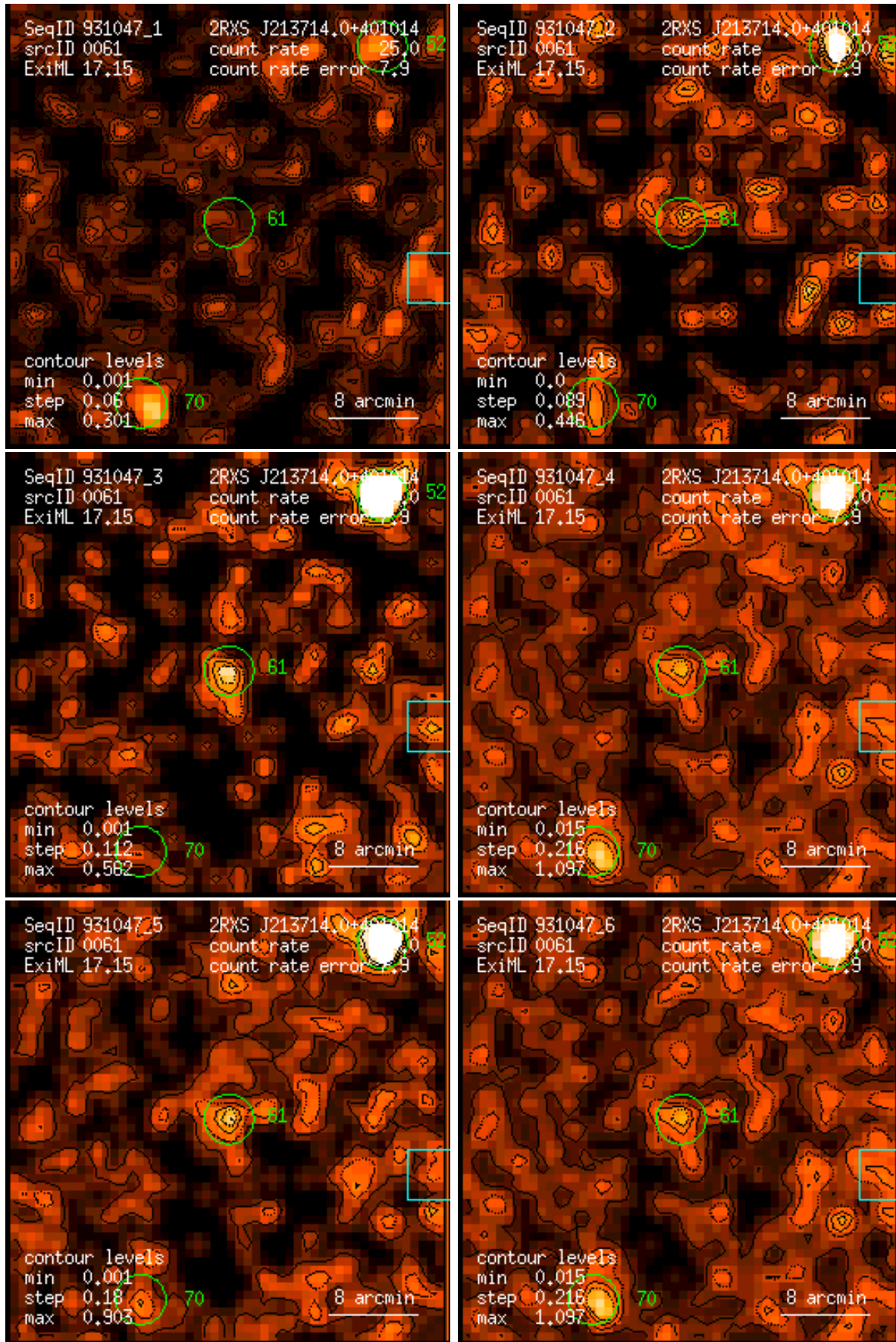
Figure 61: RASS 931047: detection 0061: band rate images, Gaussian filter: (1) PSPC channels 11 – 41, (2) 52 – 90, (3) 91 – 201, (4) 11 – 235, (5) 52 – 201, (6) 11 – 201. Broad band rates in counts/ks. Band rate contour levels in counts/ks/arcmin 2 .
