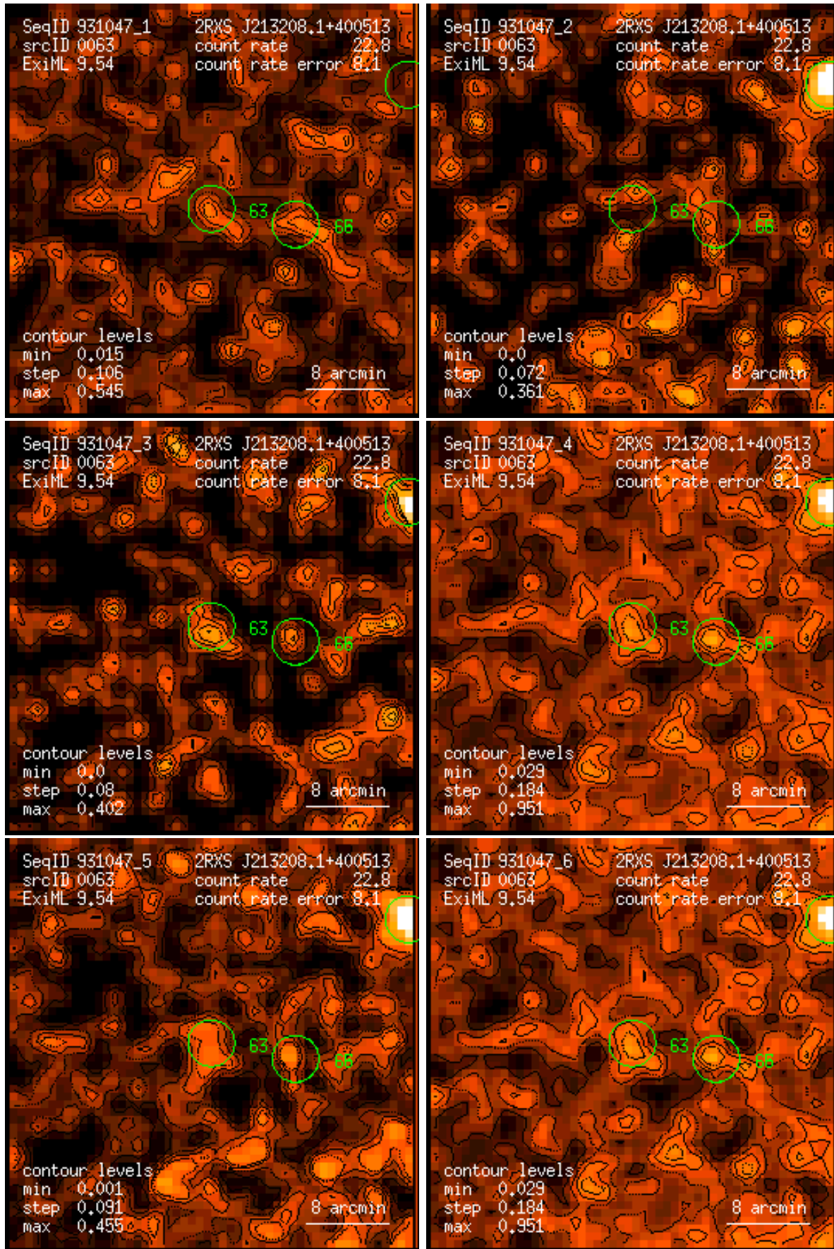
Figure 63: RASS 931047: detection 0063: band rate images, Gaussian filter: (1) PSPC channels 11 – 41, (2) 52 – 90, (3) 91 – 201, (4) 11 – 235, (5) 52 – 201, (6) 11 – 201. Broad band rates in counts/ks. Band rate contour levels in counts/ks/arcmin 2 .
