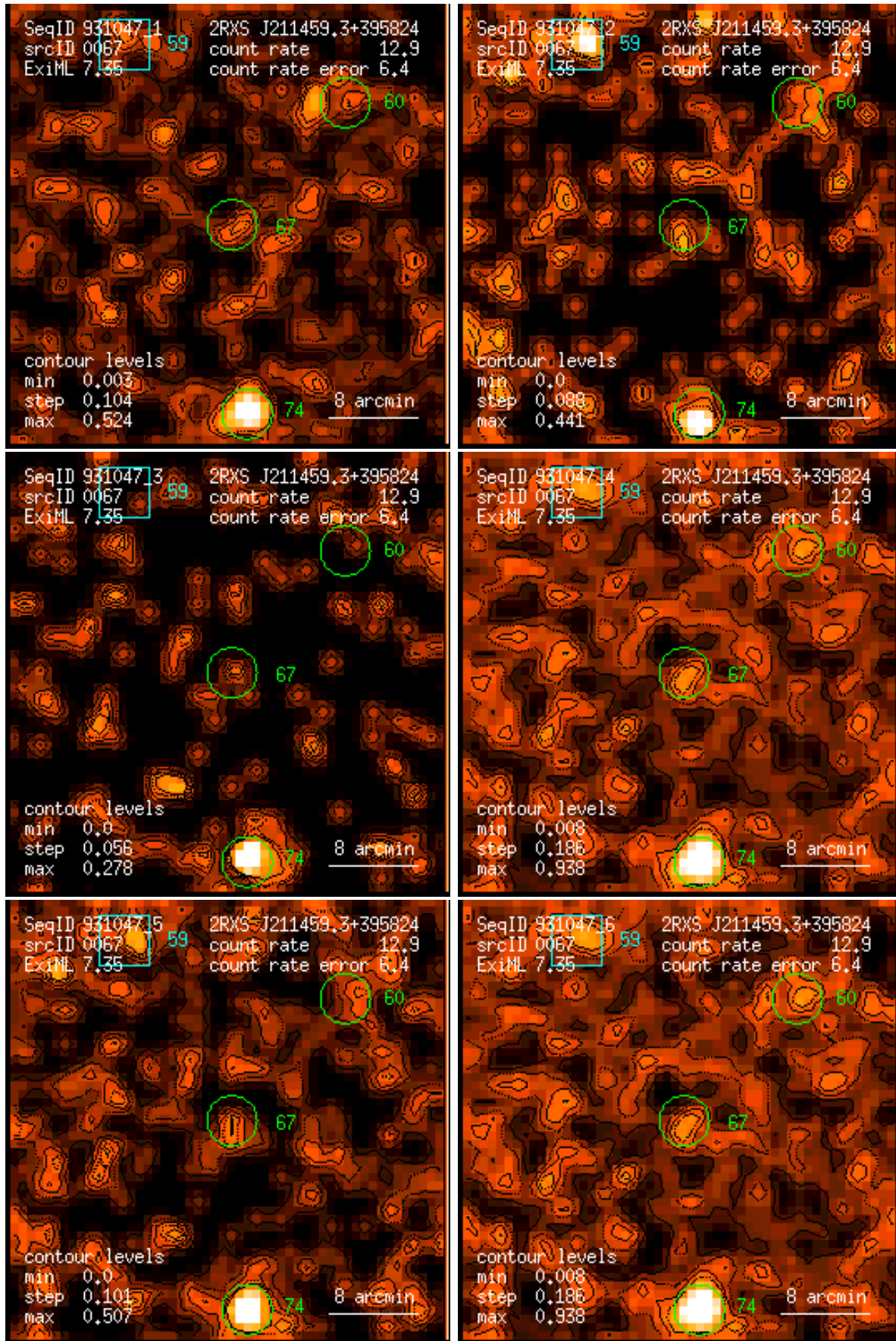
Figure 67: RASS 931047: detection 0067: band rate images, Gaussian filter: (1) PSPC channels 11 – 41, (2) 52 – 90, (3) 91 – 201, (4) 11 – 235, (5) 52 – 201, (6) 11 – 201. Broad band rates in counts/ks. Band rate contour levels in counts/ks/arcmin 2 .
